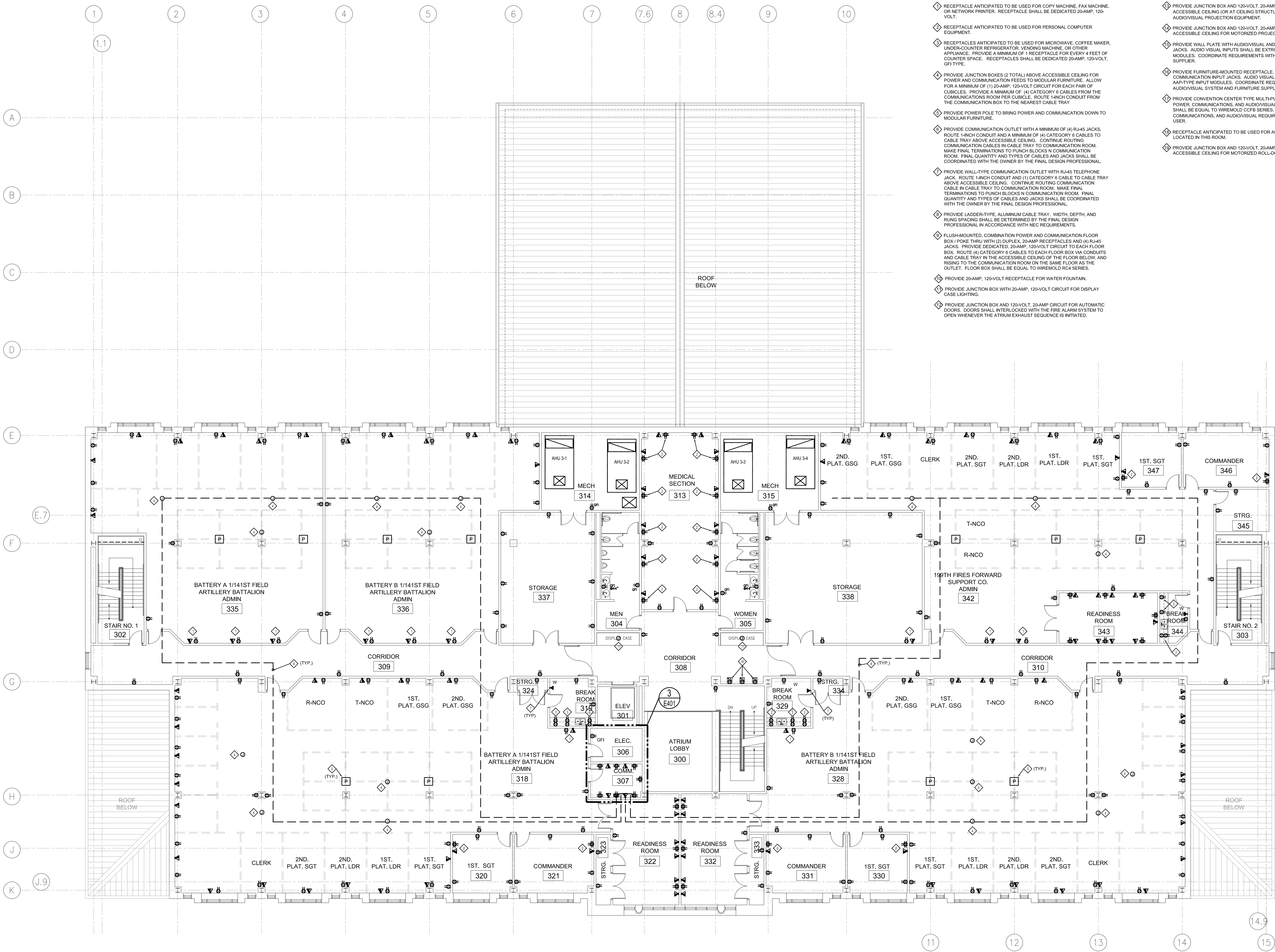
1 POWER/COMMUNICATION PLAN - THIRD FLOOR SCALE 1/8" = 1'-0" PROJECT NORTH TRUE NORTH
