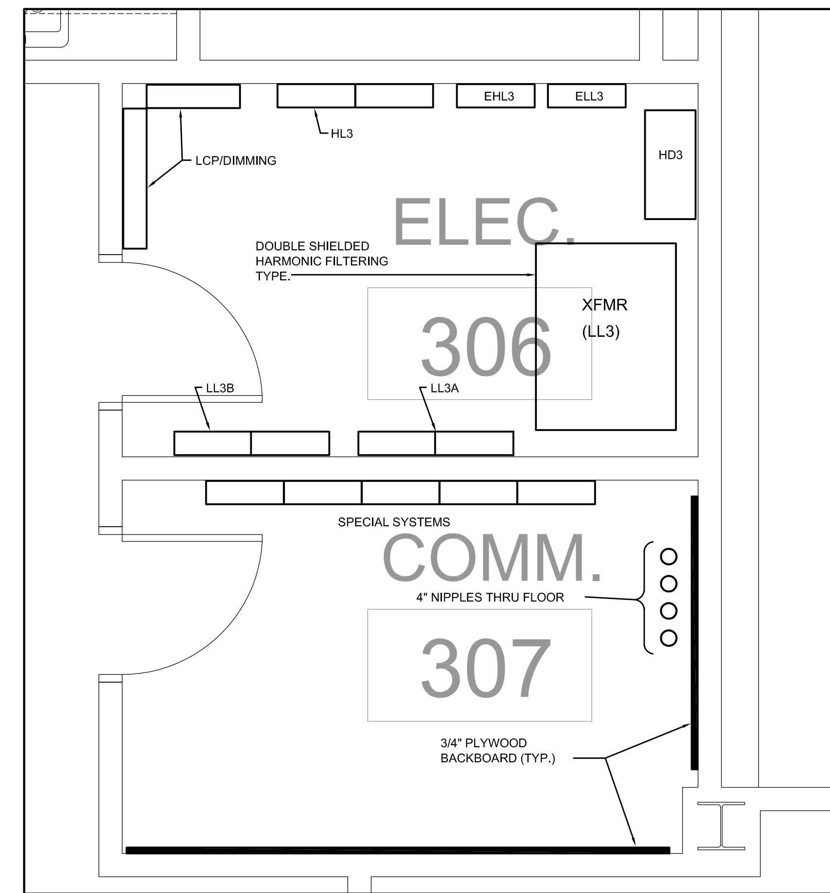
3 THIRD FLOOR ENLARGED ELECTRICAL PLAN SCALE: 1/2"=1'-0"
