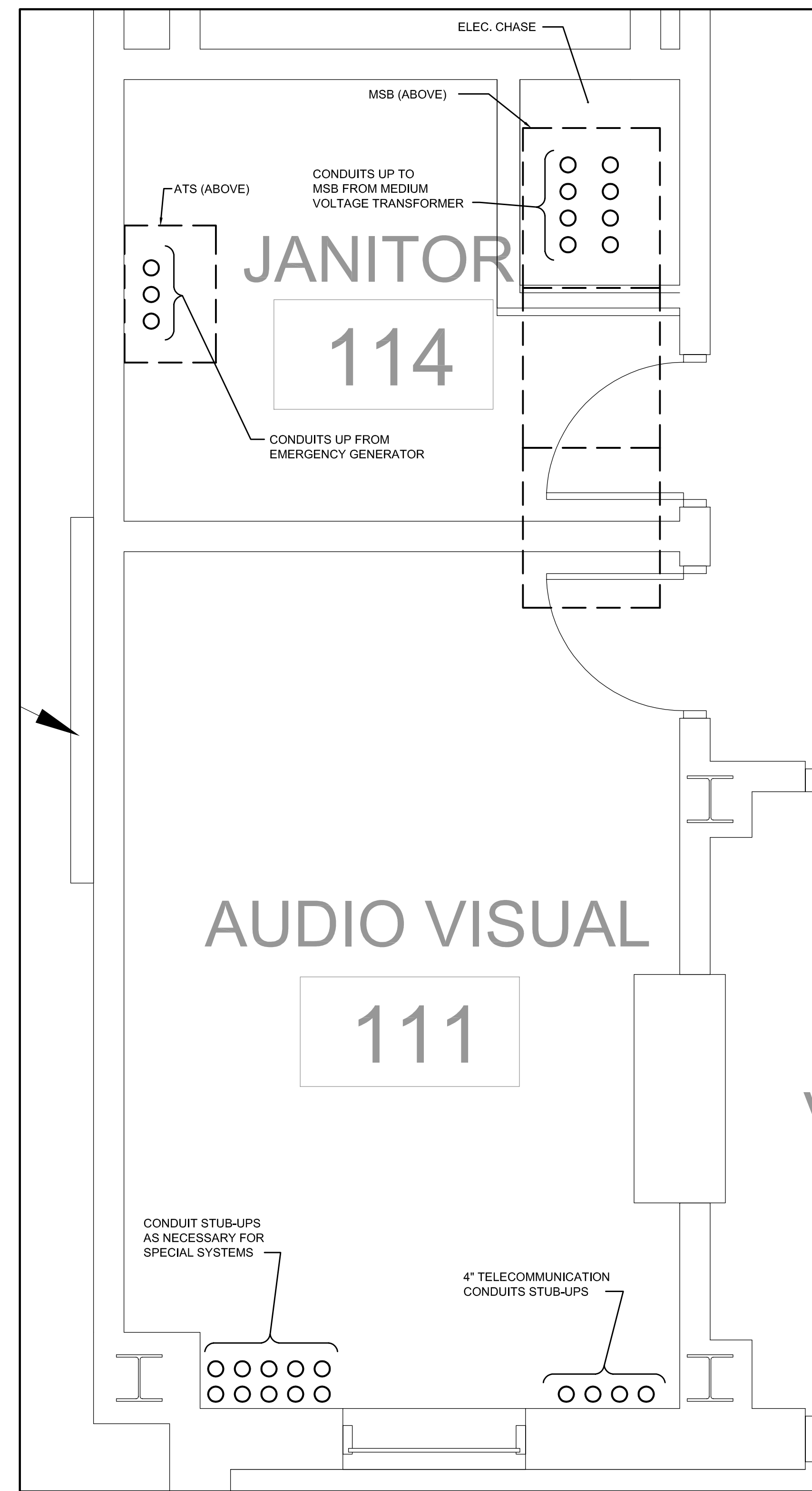
1 FIRST FLOOR ENLARGED ELECTRICAL PLAN SCALE: 1/2"=1'-0"
