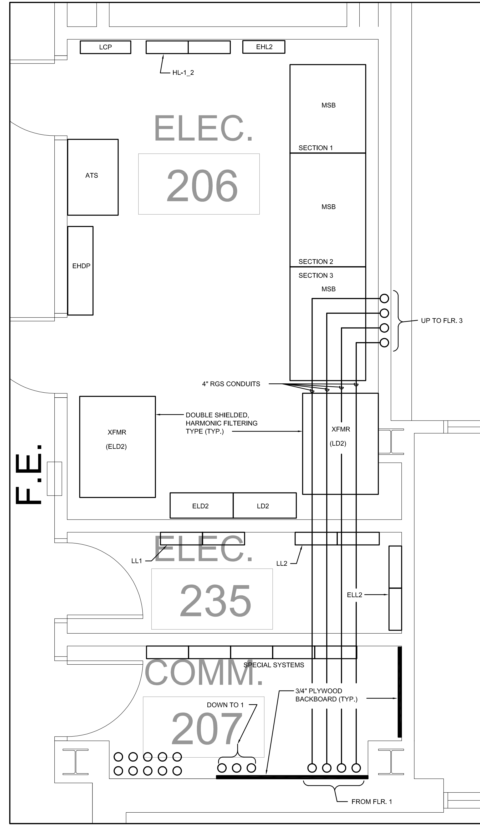
2 SECOND FLOOR ENLARGED ELECTRICAL PLAN SCALE: 1/2"=1'-0"
