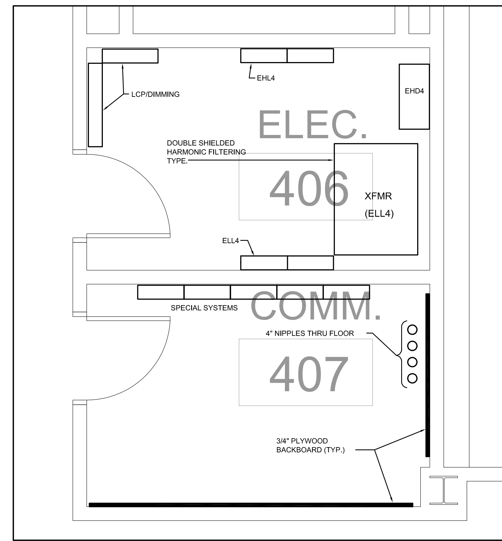
4 FOURTH FLOOR ENLARGED ELECTRICAL PLAN SCALE: 1/2"=1'-0"
