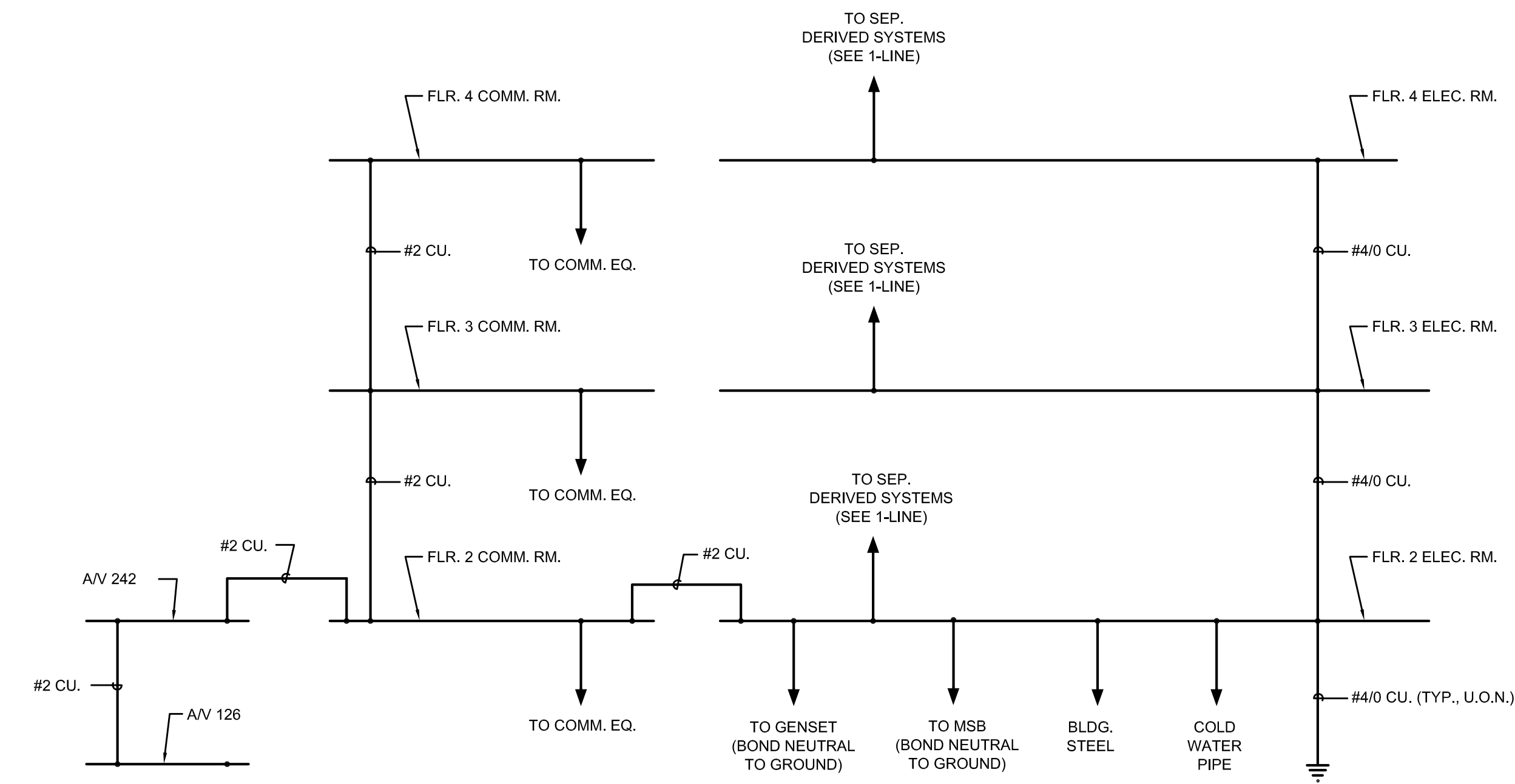
2 GROUNDING SYSTEM RISER SCALE: NTS
