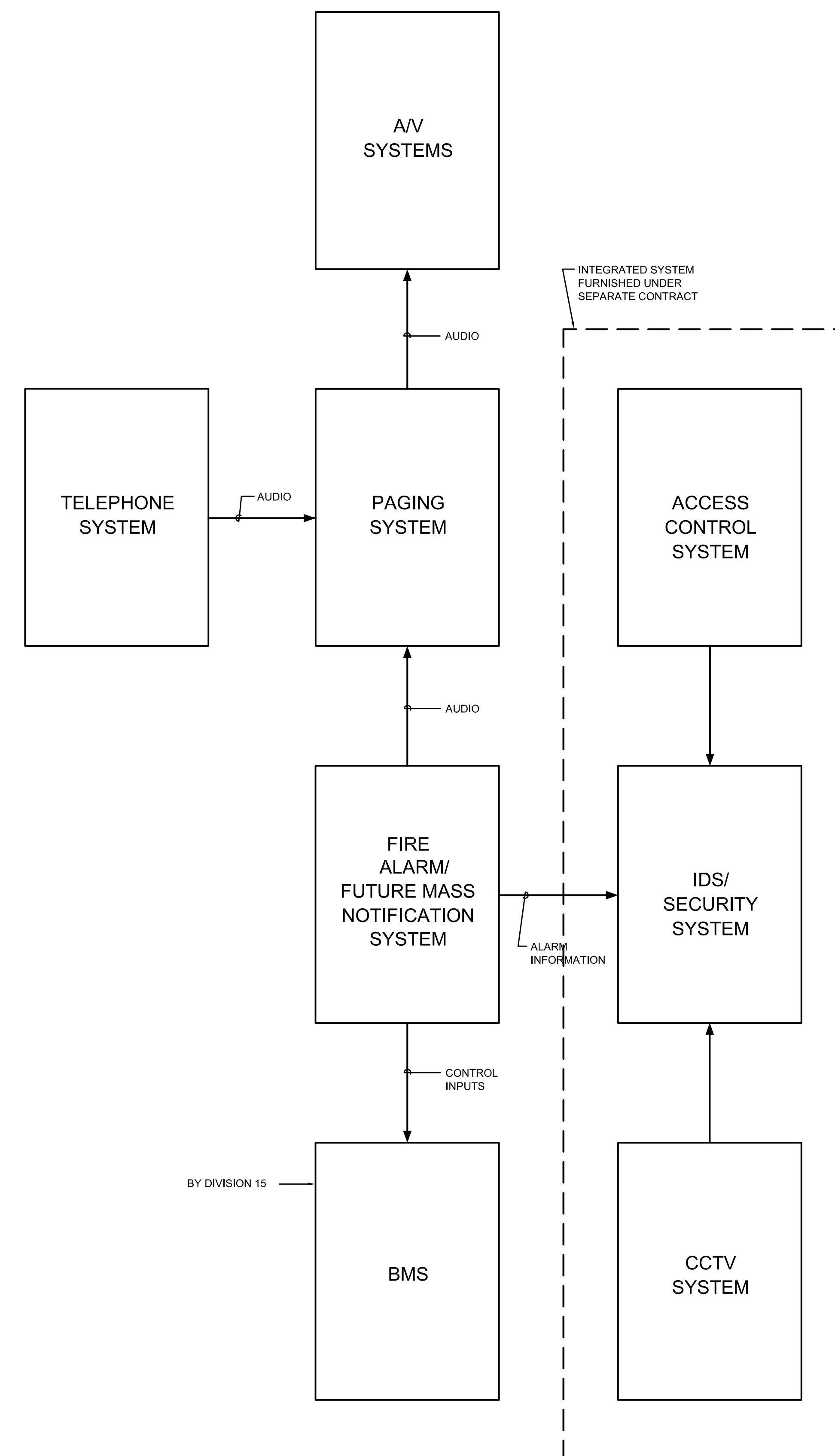
3 BLOCK DIAGRAM - SPECIAL SYSTEM INTERCONNECTIONS SCALE: NTS
