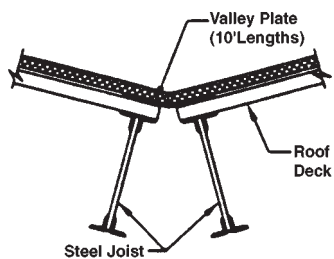
VALLEY DETAIL
