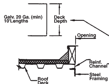
REINFORCING CHANNEL
