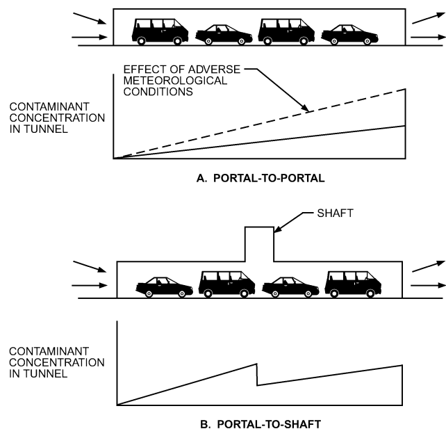
Fig. 2 Natural Ventilation
