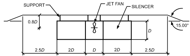
Fig. 24 Typical Jet Fan Arrangement in Niche
