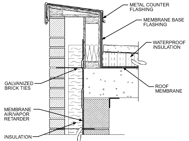
Fig. 3 Detail of Concrete Roof Deck with Continuous Wall/Room Airflow Retarder
