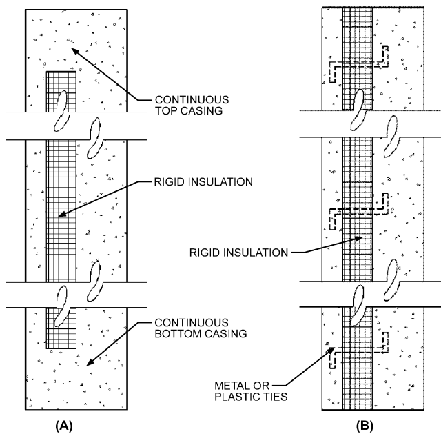
Fig. 7 Sandwich Panel with Insulation Encased in Concrete
