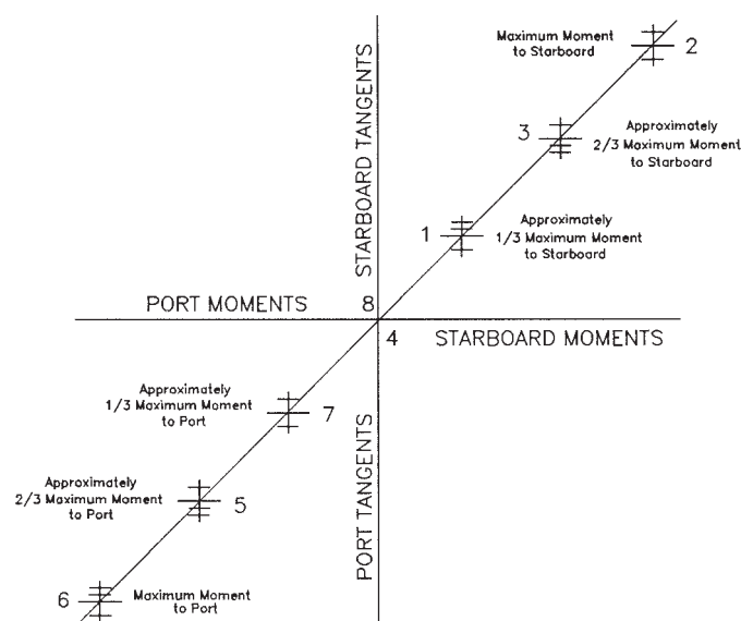
FIG. 18 Acceptable Spread of Test Points On Incline Plot
