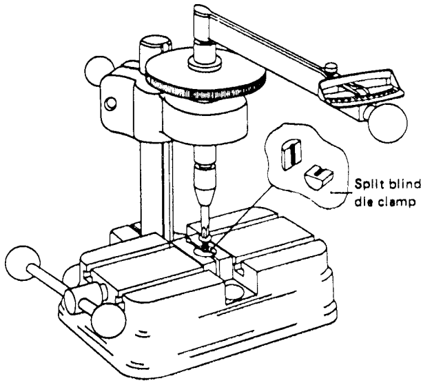
FIG. 2 Torque-Measuring Device
