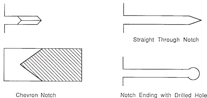
FIG. 5 Fatigue Crack Starter Notch Configurations
