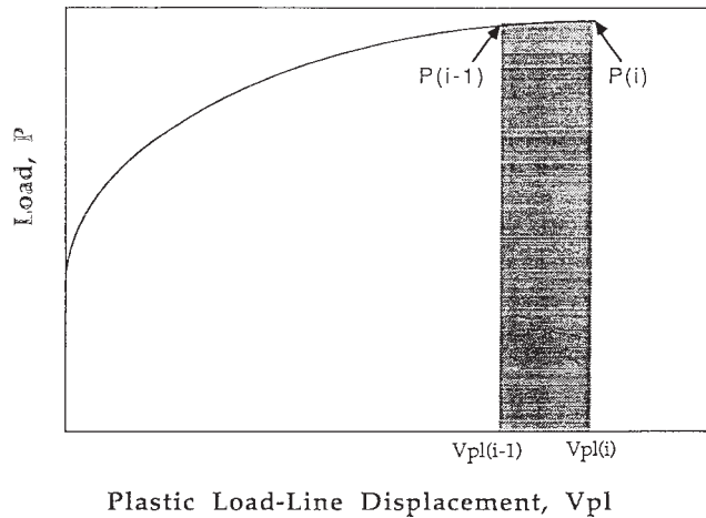
FIG. A1.3 Definition of Plastic Area for Resistance Curve J Calculation
