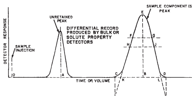
FIG. 2 Typical Chromatogram
