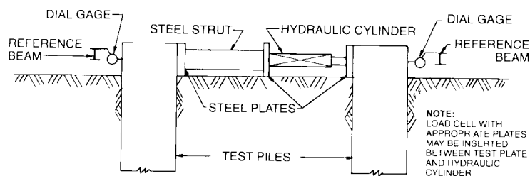
FIG. 2 Typical Arrangement for Testing Two Piles Simultaneously
