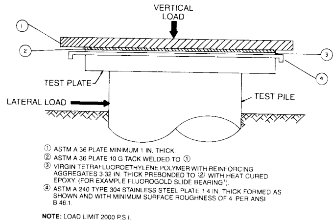
(b) ANTIFRICTION PLATE ASSEMBLY
