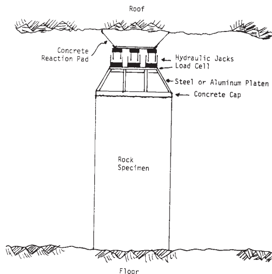
FIG. 2 Test Arrangement
