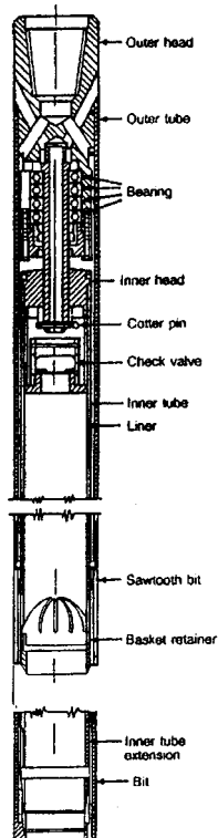
FIG. 8 Denison Sampler in Soil Sampling Configuration With Inner Core Barrel Ahead of Rotating Sawtooth Bit (23)
