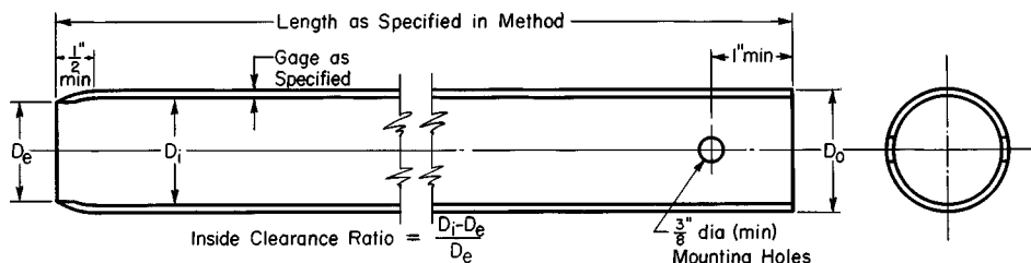
FIG. 4 Thin-Wall Sampler (see Practice D 1587)
