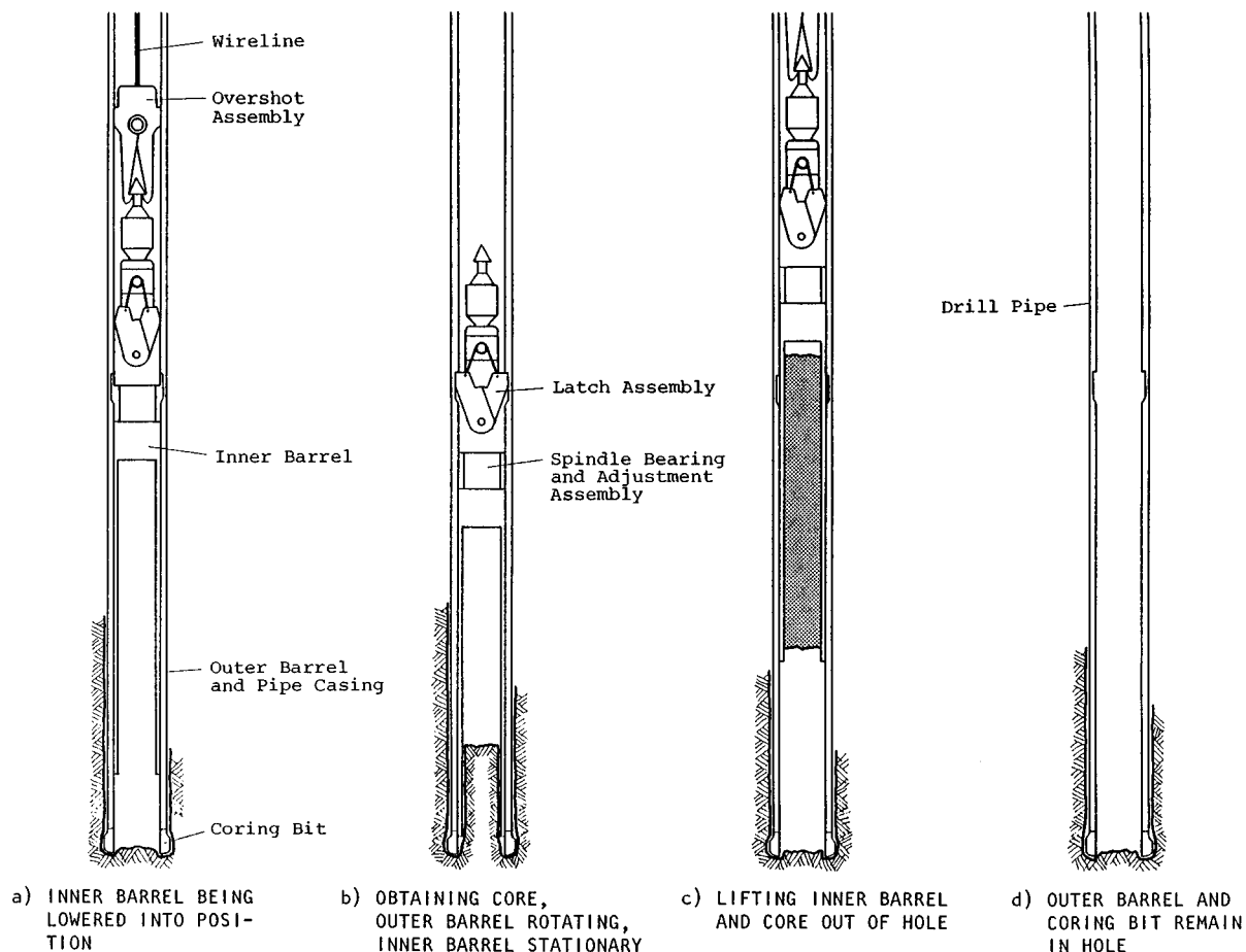
FIG. 1 Operating Principle of Wireline Core Barrel (20)
