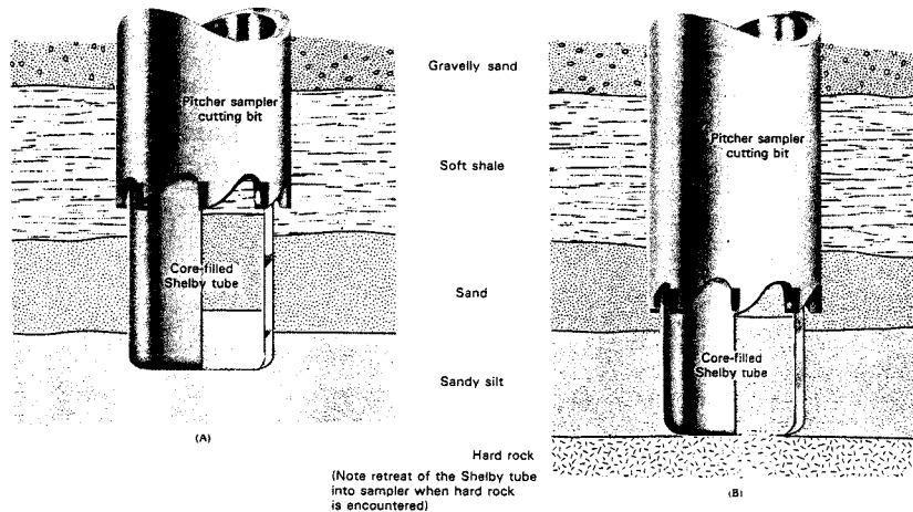
FIG. 7 Pitcher Sampler Operation: Inner Thin-Wall Barrel Extends Beyond Cutting Bit in Soft Formations (A) and Retracts into Cutting Barrel When Dense Formation is Encountered (B) (7)
