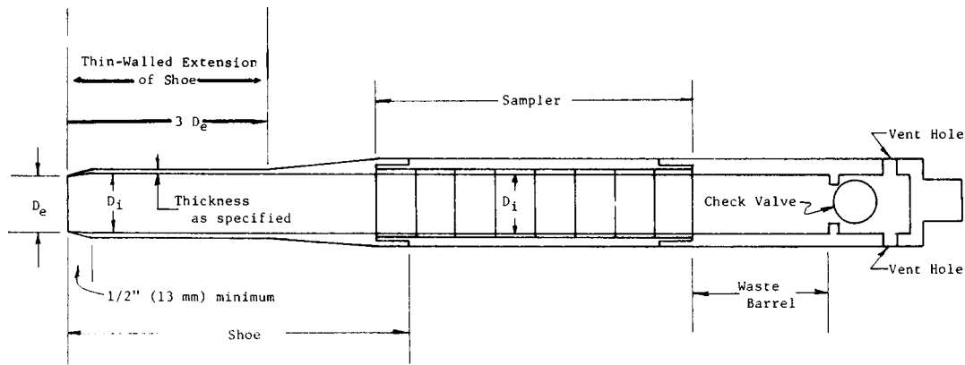
FIG. 3 Ring-Line Sampler (see Practice D 3550)
