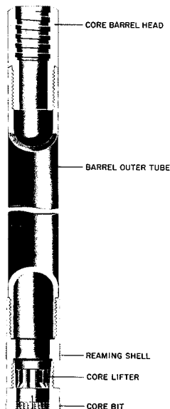
FIG. 10 G-Design Single Tube Core Barrel (25)
