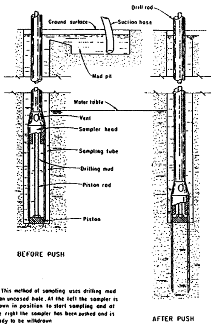
FIG. 5 Sampling With Hvorslev-Type Fixed-Piston Sampler (24)
