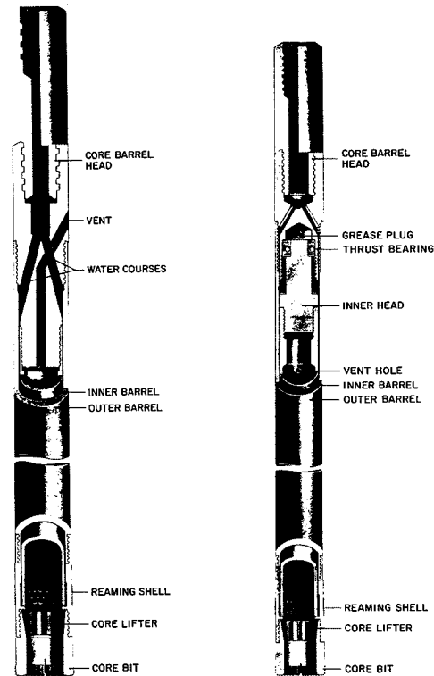
FIG. 11 G-Design Double Tube Core Barrels: (A) Rigid Type and (B) Swivel Type (25)
