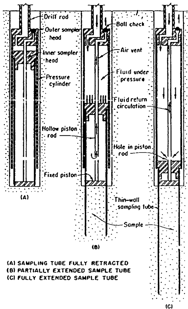
FIG. 6 Sampling With Osterberg-Type Thin-Wall Fixed-Piston Sampler (24)
