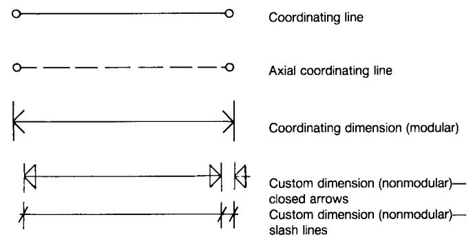
FIG. 7 Drawing Conventions with Dimensional Coordination
