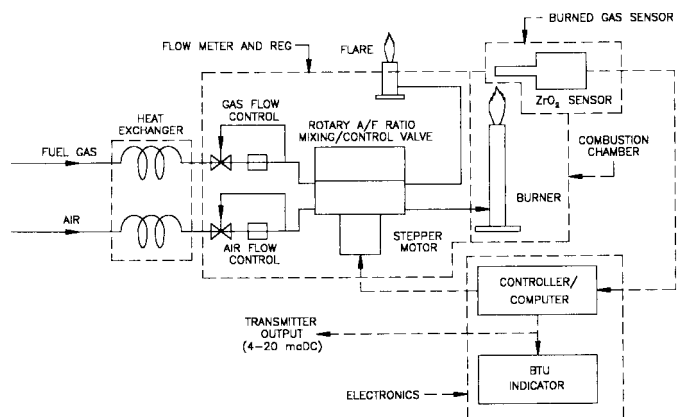
FIG. 1 Gas Btu Transmitter (Functional Overview)
