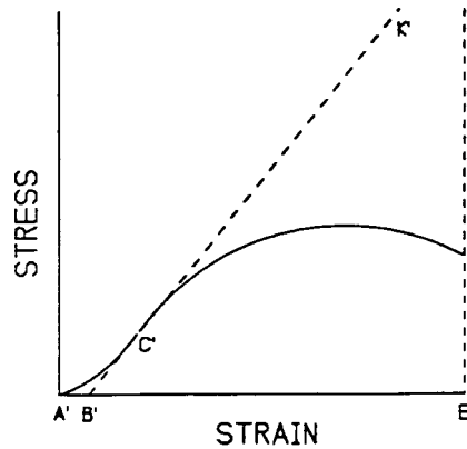
FIG. X1.2 Example of Material with No Hookean Region
