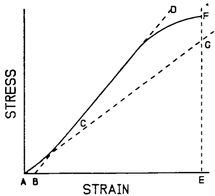
FIG. X1.1 Example of Material with Hookean Region
