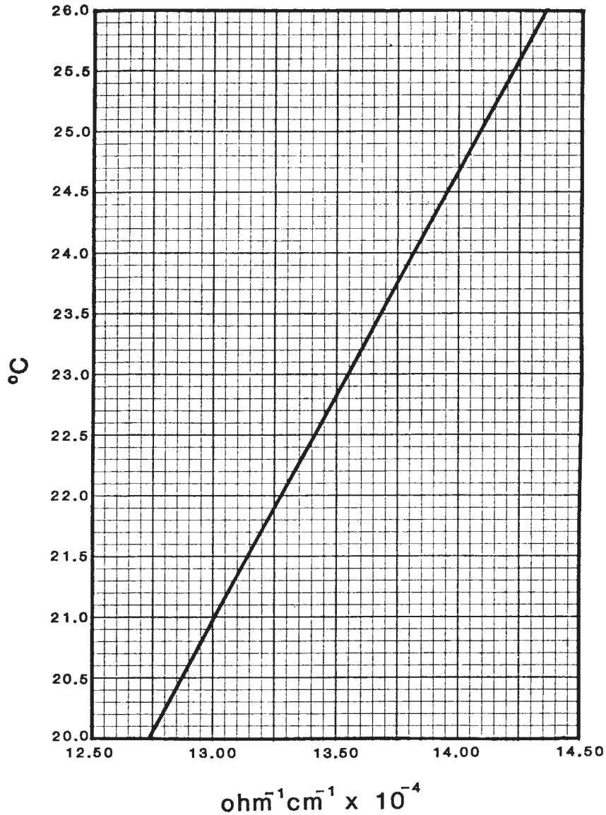
FIG. 1 Specific Conductance of 0.0100 Demal KCl
