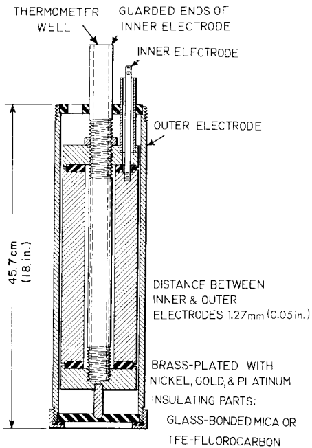
FIG. A3.1 Measuring Cell for Resistivity, Dissipation Factor, and Dielectric Constant Determinations
