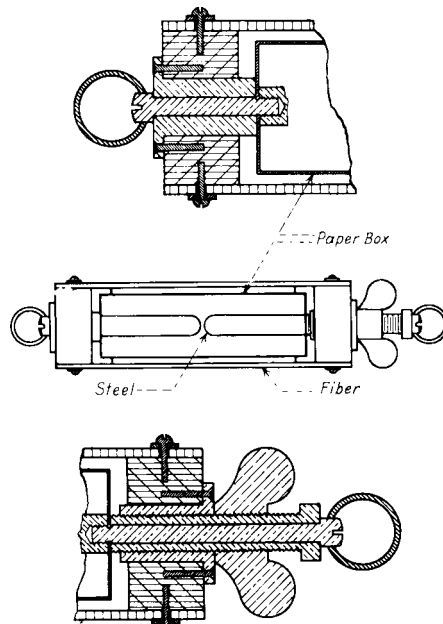
FIG. A2.1 Container for Dielectric Strength Test Showing Electrodes in Place
