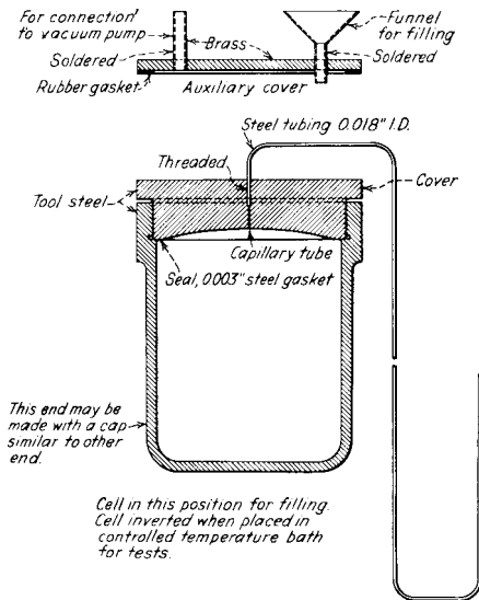
FIG. A1.1 Metallic Cell for Coefficient of Expansion Determinations
