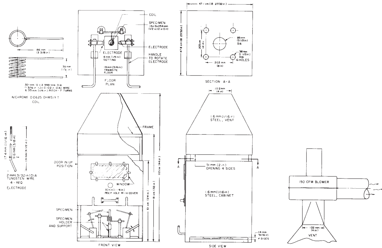
FIG. 5 Flame Cabinet
