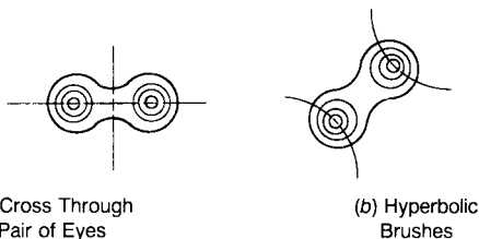
FIG. X1.1 Diagrams in Measuring Optical Axial Angle of Mica
