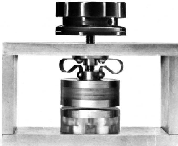
FIG. X1.2 Test Electrodes
