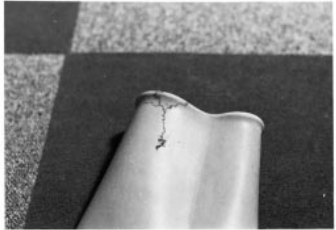
FIG. 25 Tracking—Insufficient Immersion Depth
