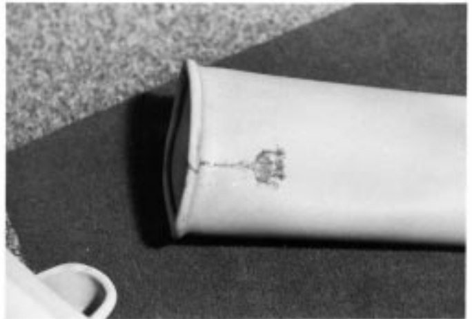
FIG. 26 Tracking—Contaminated Dielectric Fluid
