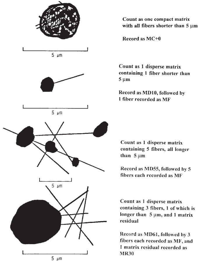
FIG. A3.3 Examples of Recording Complex Asbestos Matrices
