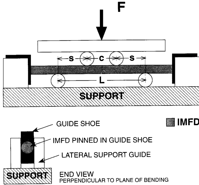
FIG. A1.2 Four-Point Bend Test with Guide Shoes
