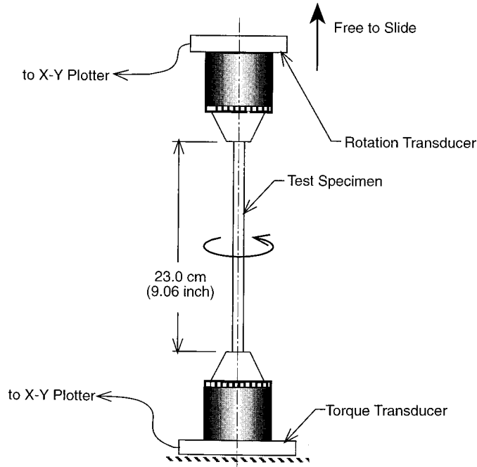
FIG. A2.1 Torsional Load Frame Setup
