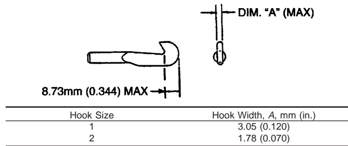
FIG. 2 Dimensions of Extractor Hook
