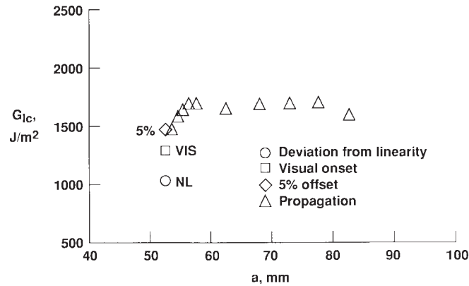
FIG. 2 Delamination Resistance Curve (R-c Curve) from DCB Test
