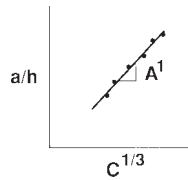
FIG. 6 Modified Compliance Calibration
