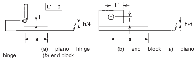
FIG. A1.1 Methods for Introducing Opening Load to DCB Specimen
