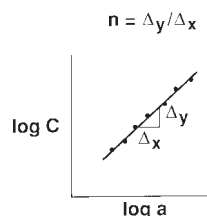
FIG. 5 Compliance Calibration
