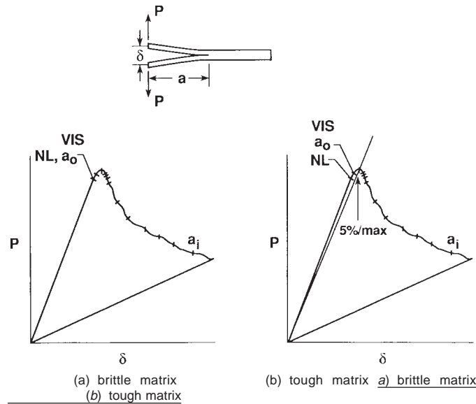
FIG. 3 Load Displacement Trace from DCB Test
