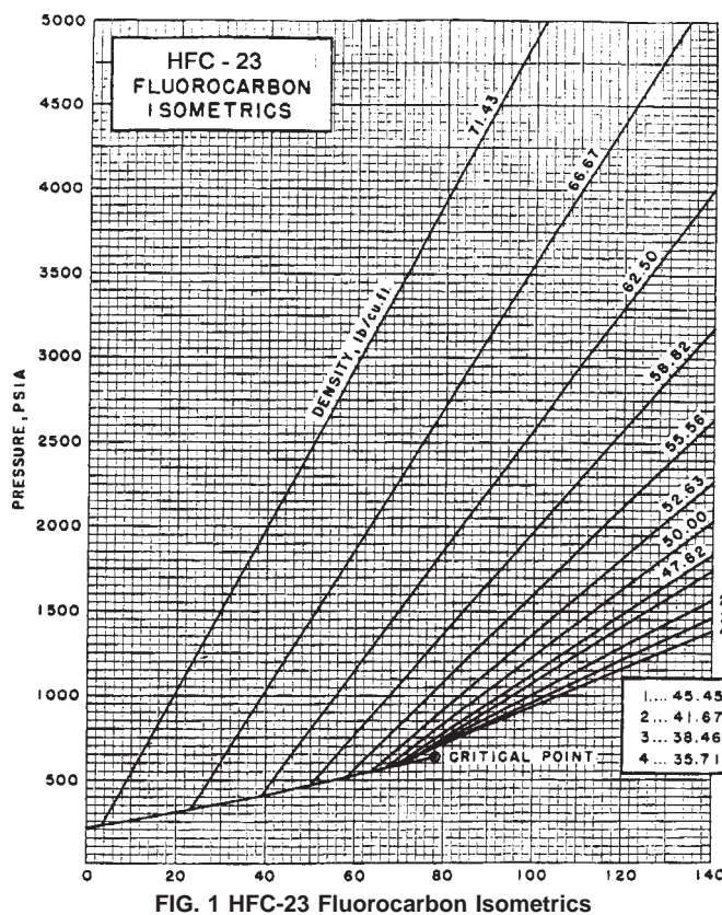
FIG. 1 HFC-23 Fluorocarbon Isotherms
