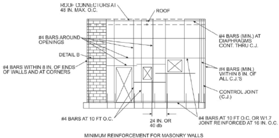
FIGURE R606.11(2) REQUIREMENTS FOR REINFORCED GROUTED MASONRY CONSTRUCTION IN SEISMIC DESIGN CATEGORY C
