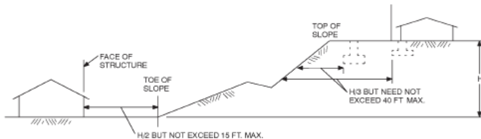
FIGURE R403.1.7.1 FOUNDATION CLEARANCE FROM SLOPES
