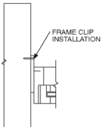
FIGURE R613.8(2) FRAME CLIP
