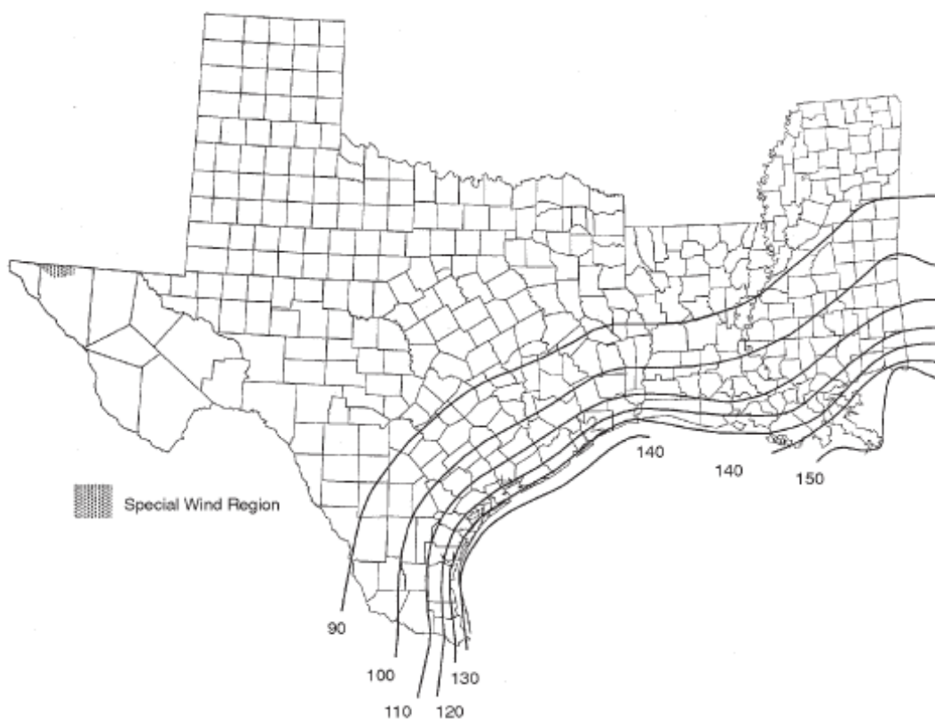
FIGURE R301.2(4)—continued BASIC WIND SPEEDS FOR 50-YEAR MEAN RECURRENCE INTERVAL
