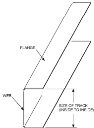
FIGURE R505.2(2) TRACK SECTION
