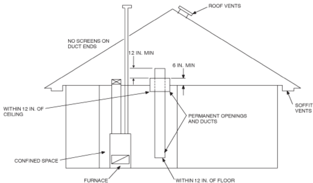
FIGURE M1703.3 APPLIANCES LOCATED IN CONFINED SPACES—ALL AIR TAKEN FROM OUTDOORS THROUGH VENTILATED ATTIC, INLET DUCT WITHIN OUTLET DUCT
