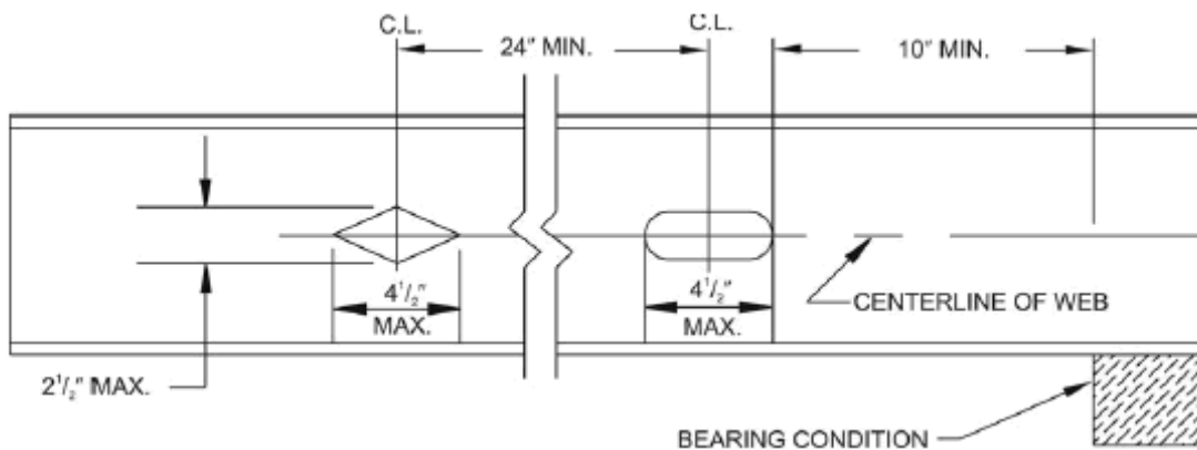
FIGURE R505.2(3) FLOOR JOIST WEB HOLES
