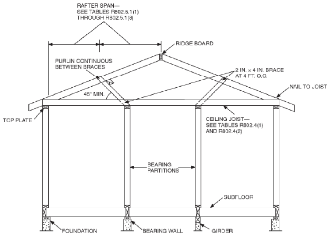
FIGURE R802.5.1 BRACED RAFTER CONSTRUCTION
