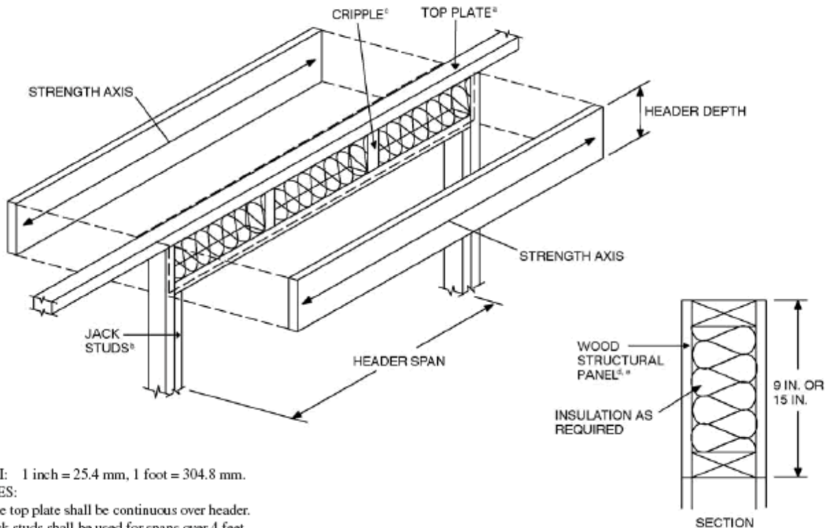
FIGURE R602.7.2 TYPICAL WOOD STRUCTURAL PANEL BOX HEADER CONSTRUCTION
