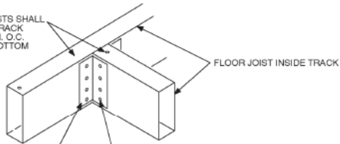
BUILT-UP HEADER OR TRIMMER JOIST
