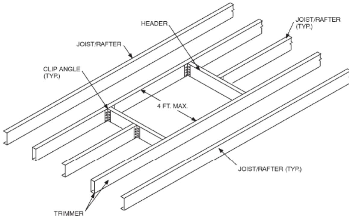
FIGURE R804.3.10(1) ROOF OPENING
