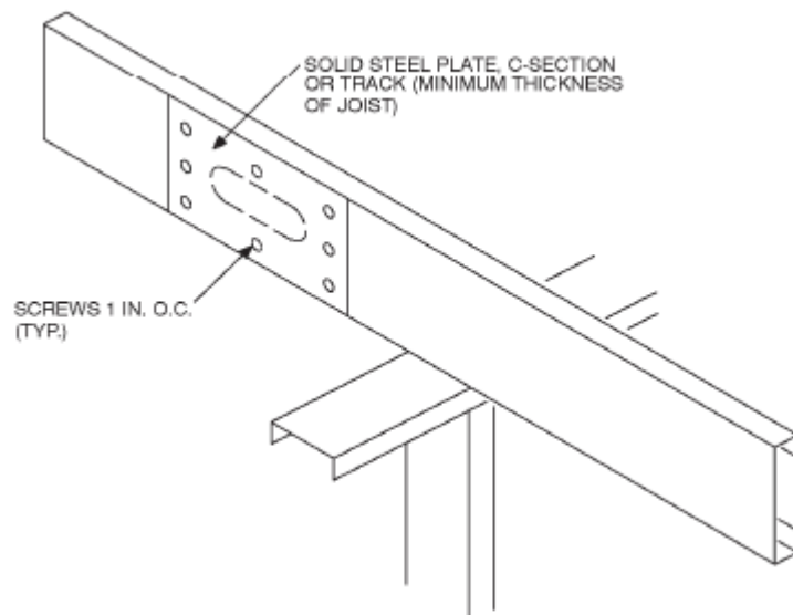
FIGURE R505.3.6 HOLE PATCH
