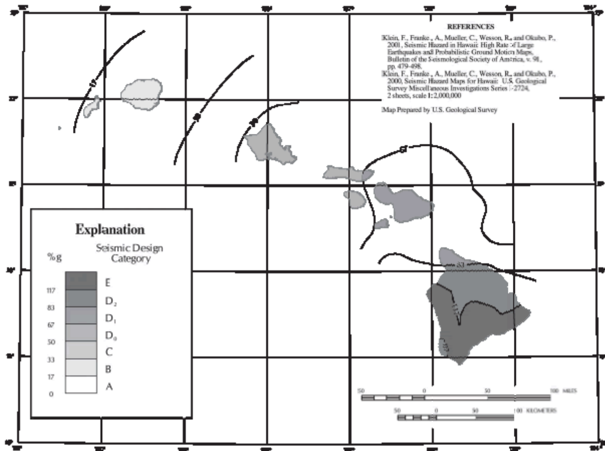
FIGURE R301.2(2)—continued SEISMIC DESIGN CATEGORIES—SITE CLASS D
