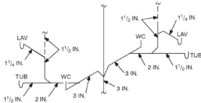
A. TYPICAL BACK-TO-BACK BATHS
