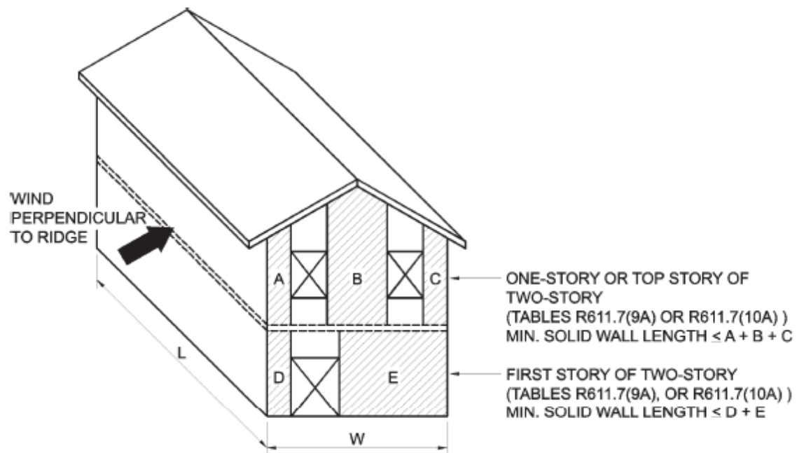
FIGURE R611.7.4 MINIMUM SOLID WALL LENGTH
