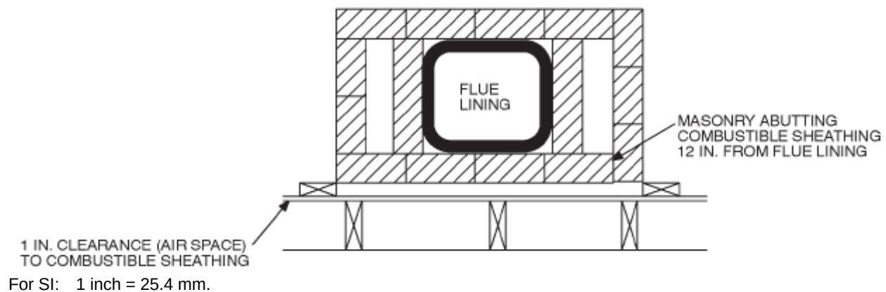
FIGURE R1003.18 CLEARANCE FROM COMBUSTIBLES
