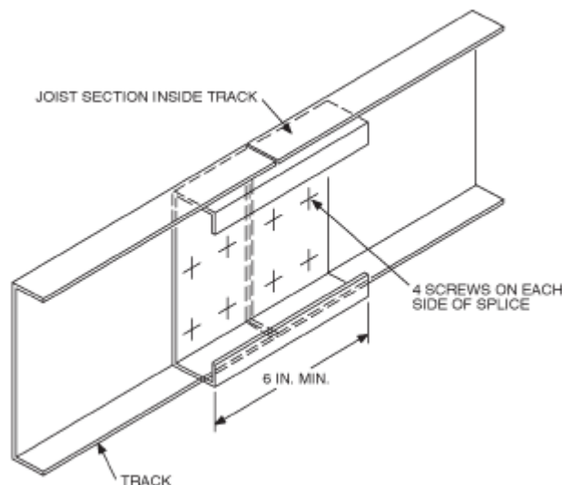
FIGURE R505.3.8 TRACK SPLICE
