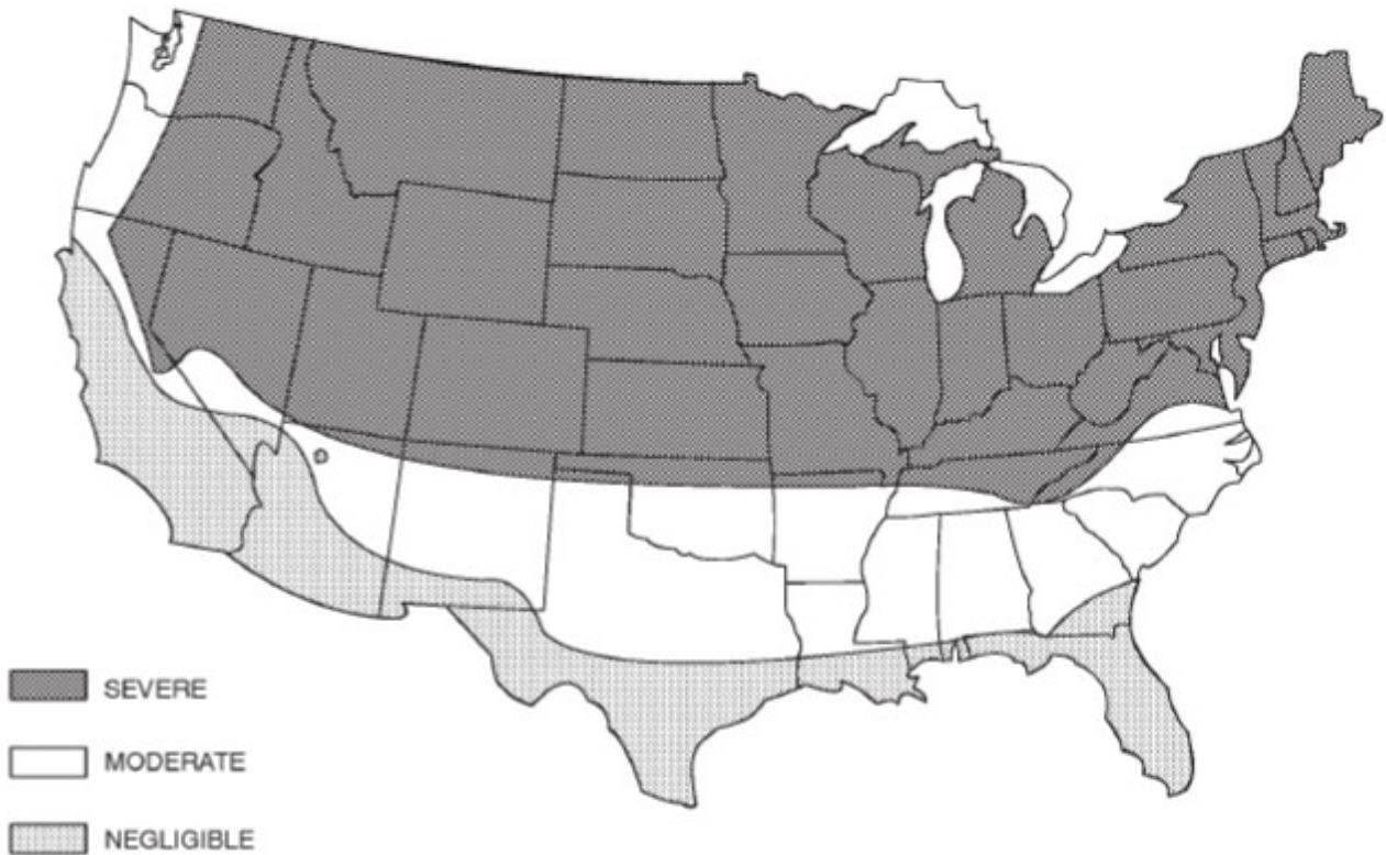
FIGURE R301.2(3) WEATHERING PROBABILITY MAP FOR CONCRETE
