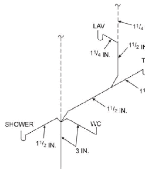
D. COMBINATION WET- AND STACK-VENTINI WITH STACK FITTING
