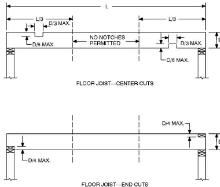
FIGURE R502.8 CUTTING, NOTCHING AND DRILLING
