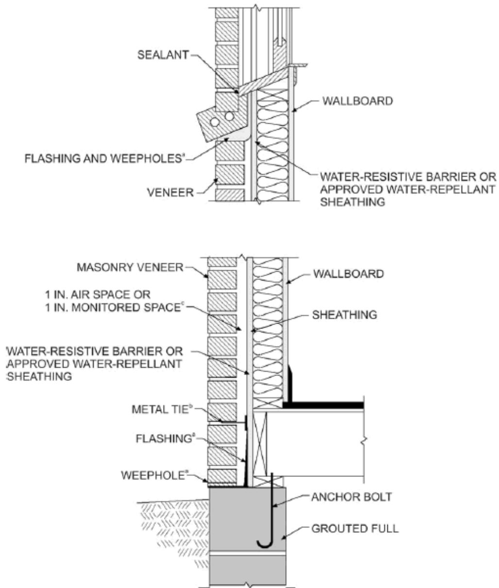
FIGURE R703.7 MASONRY VENEER WALL DETAILS
