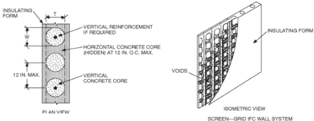
FIGURE R611.5 SCREEN-GRID IFC WALL SYSTEM
