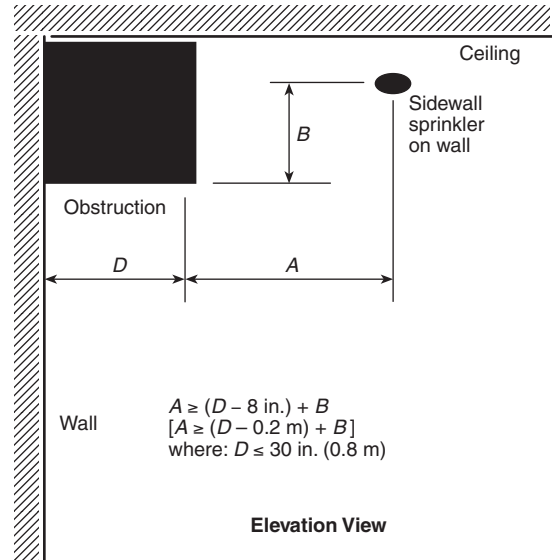
FIGURE 8.9.5.1.4(b) Obstruction Against Wall (Extended Coverage Sidewall Spray Sprinklers).
