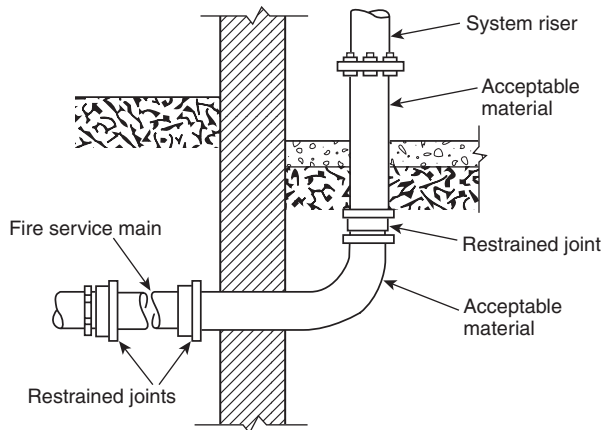
FIGURE A.10.6.2 Typical Connection to a Fire Protection System Riser Illustrating Restrained Joints. [24:Figure A.10.6.2]
