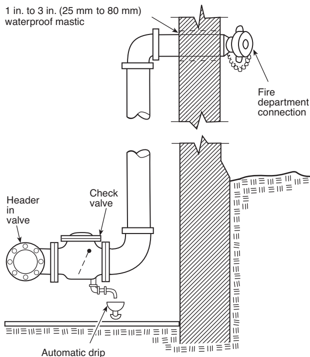
FIGURE 8.17.2.1 Fire Department Connection.
