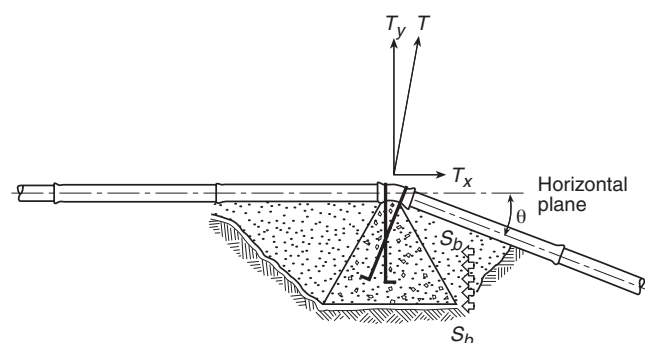
FIGURE A.10.6.1(b) Bearing Thrust Block. [24:Figure A.10.6.1(b)]
