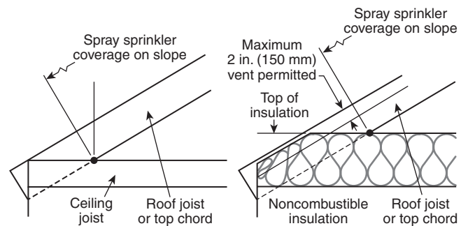
FIGURE A.8.6.4.1.4.3 Attic Width and Sprinkler Spacing Measurements.
