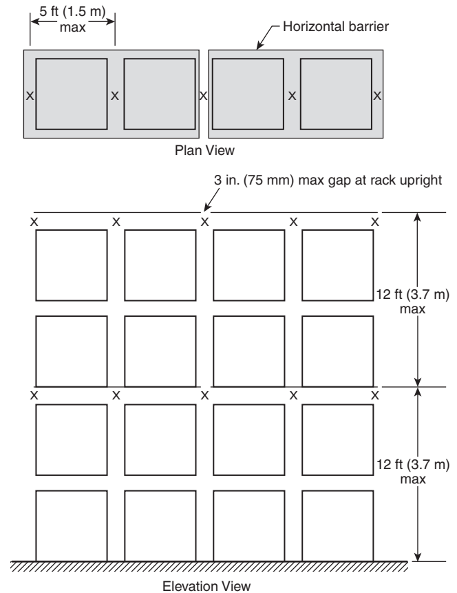
FIGURE 17.1.2.9.4.1(A) Alternative Protection Single-Row Racks.
