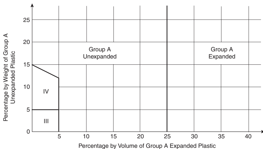
FIGURE 5.6.3.3.3(b) Exposed Commodities Containing a Mixture of Expanded and Unexpanded Group A Plastics.
