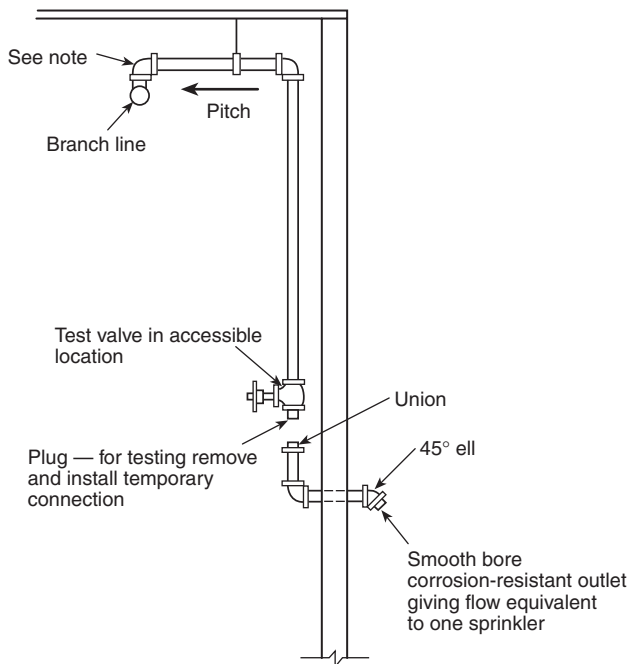
FIGURE A.8.17.5.2.2(b) Acceptable Piping Arrangement for Combined Sprinkler/Standpipe System. [14:Figure A.6.3.5(b)]
