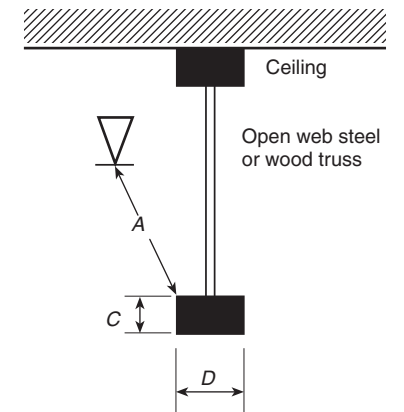
Elevation View of Truss (Obstruction in horizontal orientation) A \geq 4C or 4D A \leq 36 in. (900 mm) (Use dimension C or D, whichever is greater)
