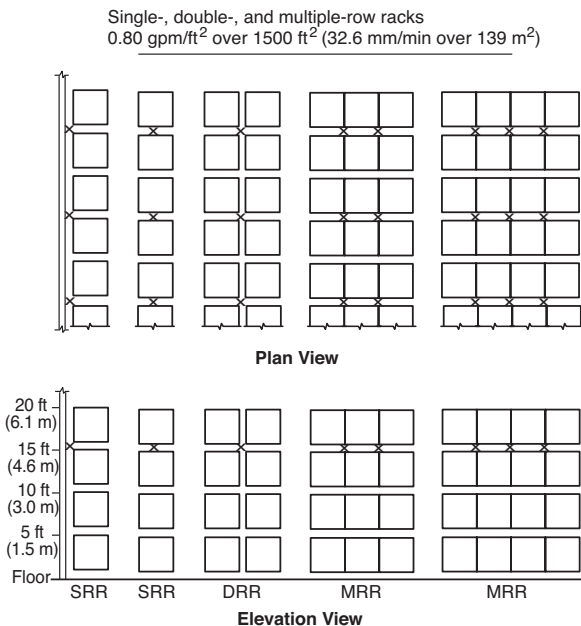
FIGURE 17.2.1.4(g) Exposed Nonexpanded Group A Plastics Up to 20 ft (6.1 m) in Height in Up to a 25 ft (7.6 m) High Building with One Level of Closely Spaced In-Rack Sprinklers.
