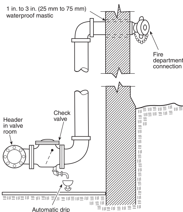
FIGURE A.8.17.2(a) Fire Department Connection.
