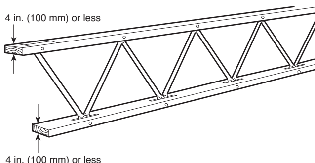
FIGURE A.3.7.2(a) Wood Bar Joist Construction.
