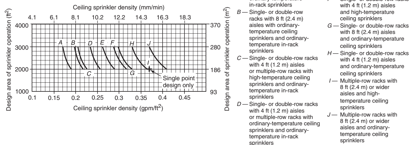
FIGURE 16.2.1.3.2(a) Sprinkler System Design Curves — 20 ft (6.1 m) High Rack Storage — Class I Nonencapsulated Commodities — Conventional Pallets.
