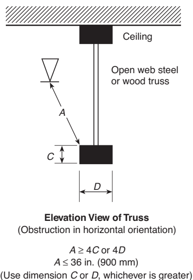
FIGURE 8.10.6.2.1.3(b) Minimum Distance from an Obstruction in the Horizontal Orientation (Residential Upright and Pendent Spray Sprinkler).
