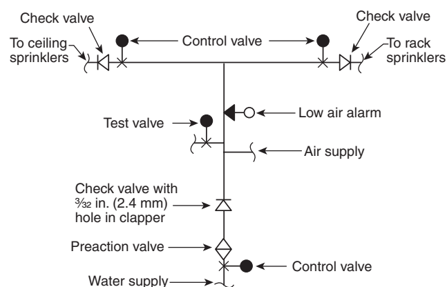
FIGURE 7.8.2.8.4 Valve Arrangement.
