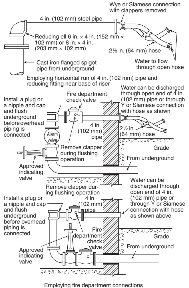
FIGURE A.10.10.2.1 Methods of Flushing Water Supply Connections. [24:Figure A.10.10.2.1]
