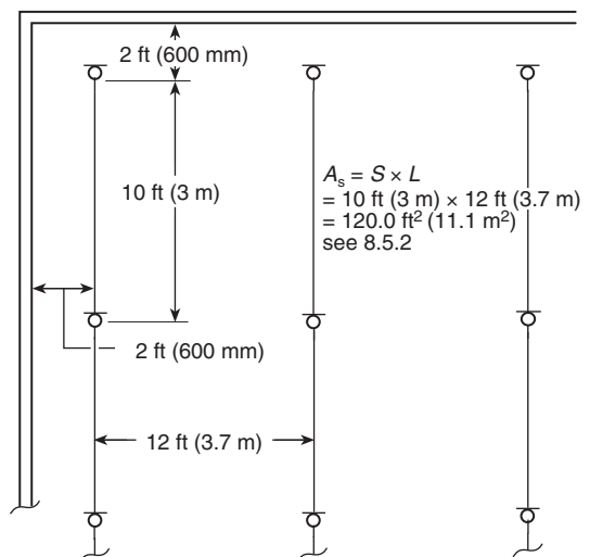
FIGURE A.23.4.4.6.2 Sprinkler Spacing.
