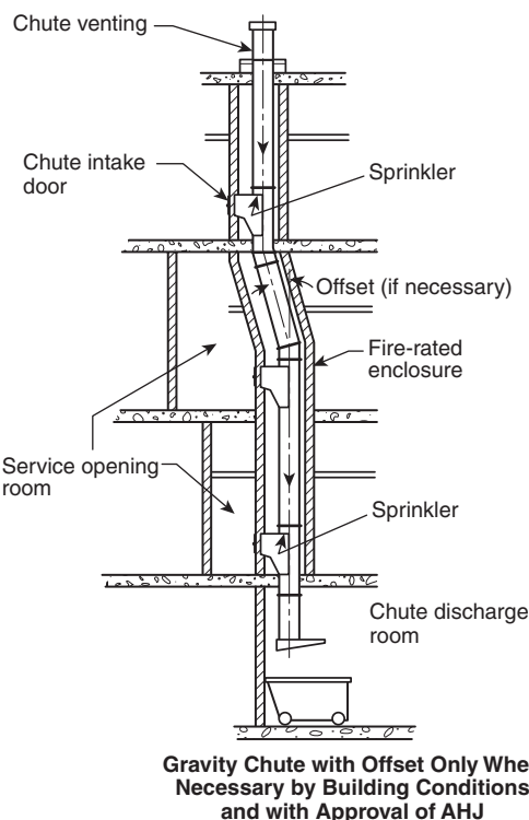
FIGURE A.22.15.2.2(b) Gravity Waste Chute. [82:Figure A.5.2(b)]
