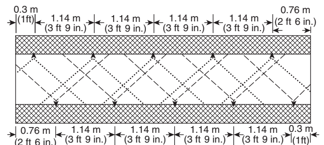
FIGURE A.22.7.1.4.6(a) Nozzle Layout for Typical Vault. [40:Figure A.6.5.6.6(a)]
