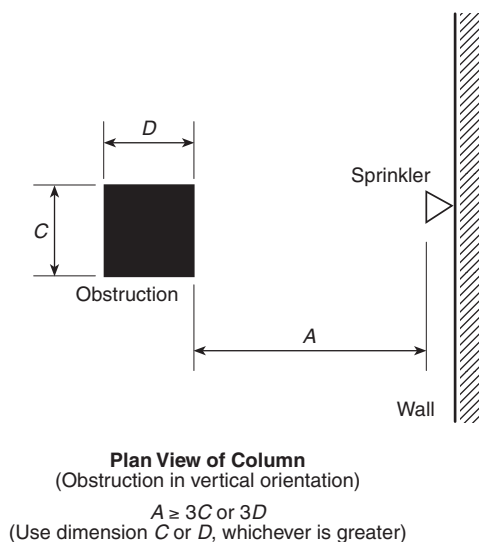
FIGURE 8.6.5.2.1.3(a) Minimum Distance from an Obstruction in the Vertical Orientation (SSU/SSP).
