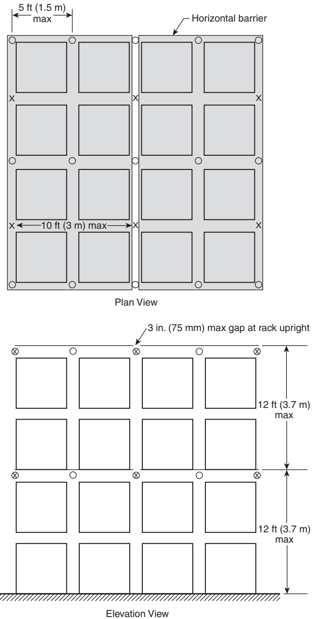
FIGURE 17.1.2.9.4.3(A) Alternative Protection Multiple-Row Racks.
