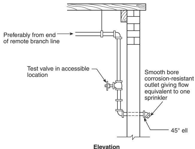
FIGURE A.8.17.4.1(a) System Test Connection on Wet Pipe System.
