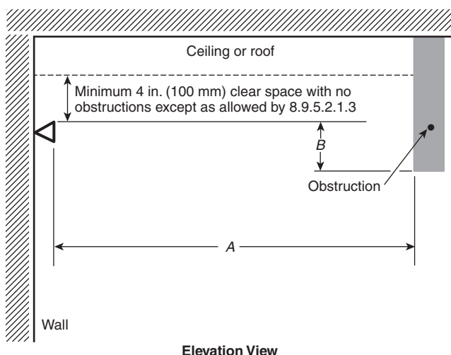
FIGURE 8.9.5.1.3 Positioning of Sprinkler to Avoid Obstruction (Extended Coverage Sidewall Spray Sprinklers).
