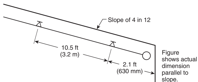
FIGURE A.23.4.4.6.5 Determination of Floor Area Under Sloped Ceiling/Roof.
