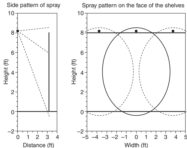
FIGURE A.22.7.1.4.4 Typical Nozzle Spray Pattern. [40:Figure A.6.5.6.4]
