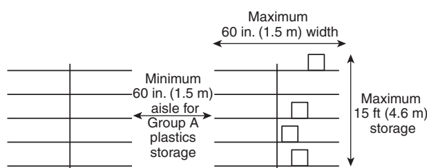
FIGURE A.3.9.2.6.1 Back-to-Back Shelf Storage.
