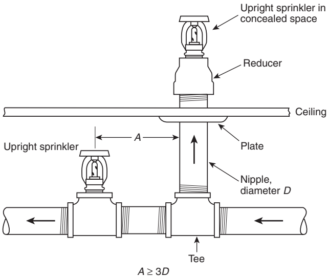
FIGURE 23.7.2.3(b) Sprinkler on Riser Nipple from Branch Line in Lower Fire Area.
