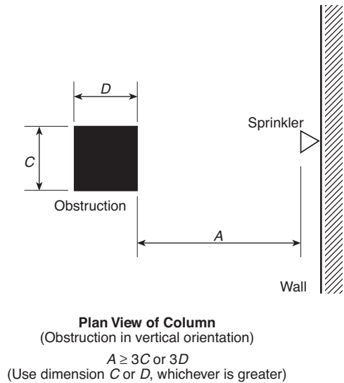
FIGURE 8.7.5.2.1.3(a) Minimum Distance from an Obstruction in the Vertical Orientation (Standard Sidewall Spray Sprinklers).
