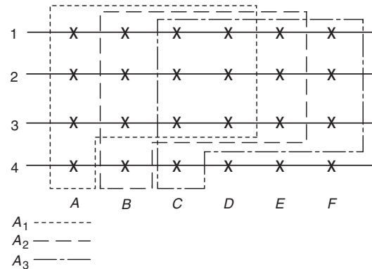
FIGURE A.23.4.4.5 Example of Determining the Most Remote Area for Gridded System.
