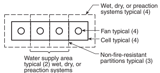
FIGURE A.22.21.1.7.2.2 Multiple Wet, Dry, or Preaction Systems with No Fire-Resistant Partitions. [214:Figure A.5.6.2.2]
