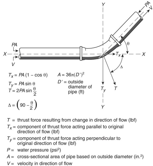
FIGURE A.10.6.1(a) Thrust Forces Acting on a Bend. [24:Figure A.10.6.1(a)]
