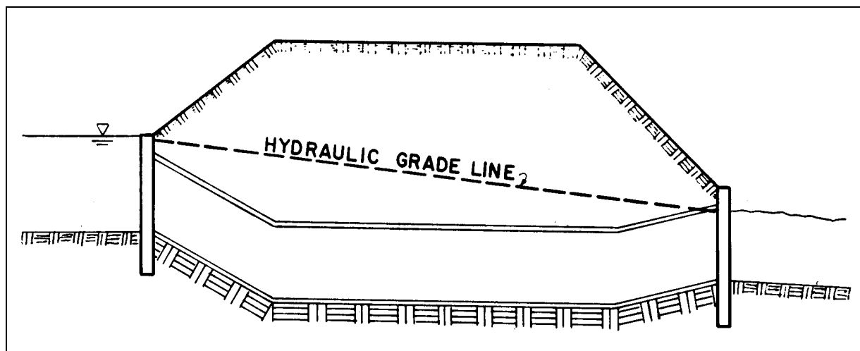
Figure VI-2--Sag Culvert
