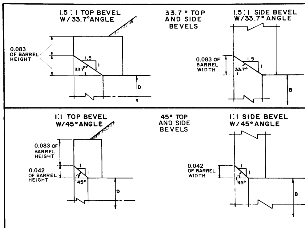
Figure III-3--Beveled Edges
