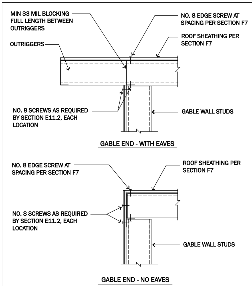
Figure E11-5 Gable Wall Roof Sheathing Attachment to Braced Walls
