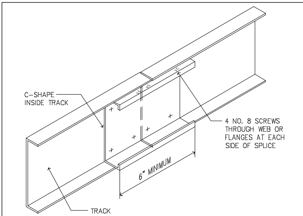
Figure D6-1 Track Splice
