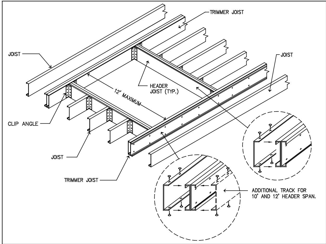
Figure D2-7 Continuous Span Joist Supported on an Interior Structural Wall
