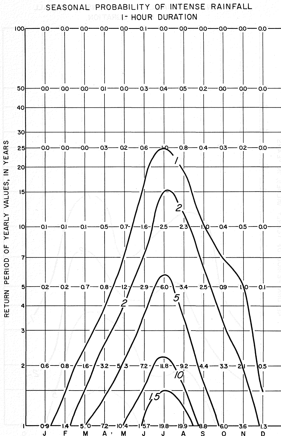
FIGURE 2-8 Probability in percent of obtaining a rainfall in any month of a particular year equal to or exceeding the yearly return period values taken from the isopluvial maps and diagrams.
