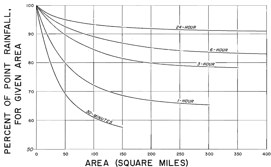
AREA-DEPTH CURVES
