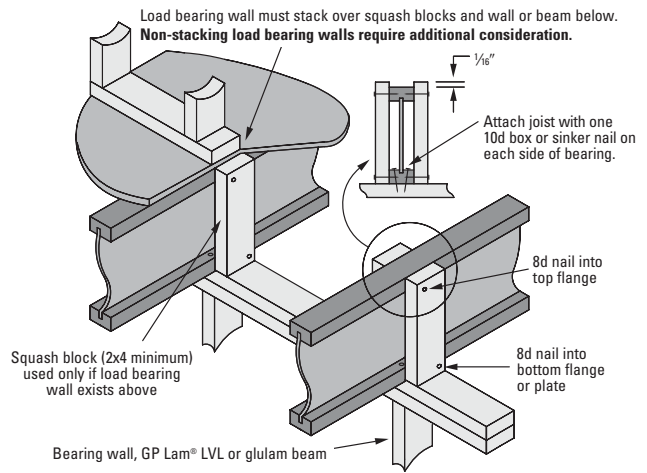
F10 SQUASH BLOCKS AT INTERIOR BEARING Vertical load transfer = 2000 plf max along load bearing wall.
