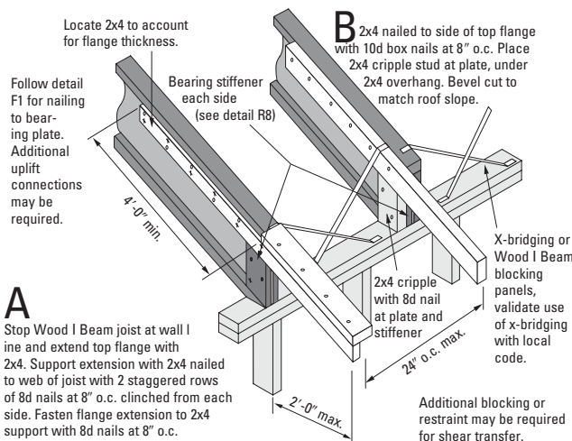
R10 OPTIONAL OVERHANG EXTENSIONS 12/12 maximum slope May be used with detail R4, R5, and R6 (Low end only)
