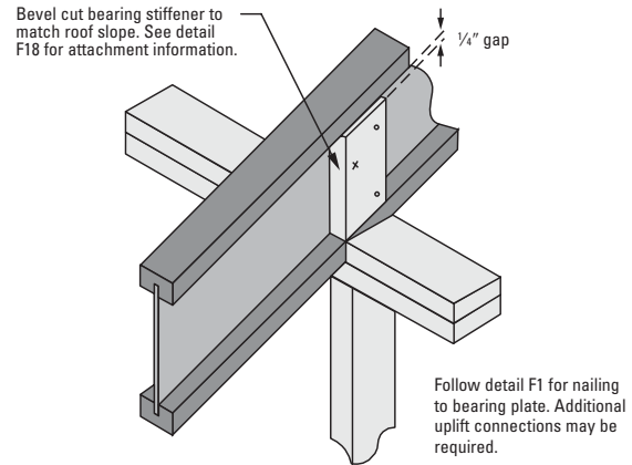
R8 BEVELED CUT BEARING STIFFENER 12/12 maximum slope
