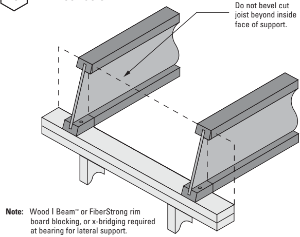
F8 BEVEL CUT JOIST
