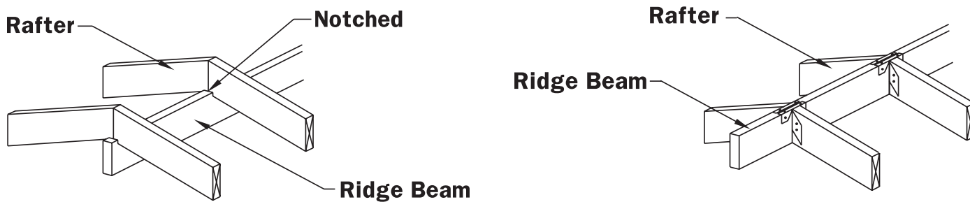
Figure 3.10a Ridge Beam Details
