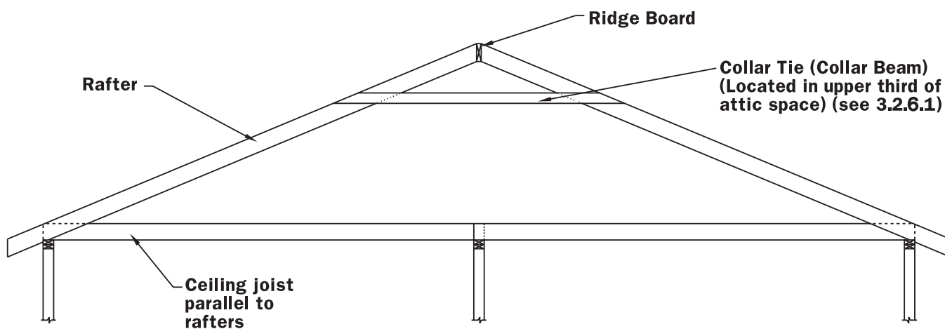
Figure 3.10b Ridge Board and Ceiling Joist Detail
