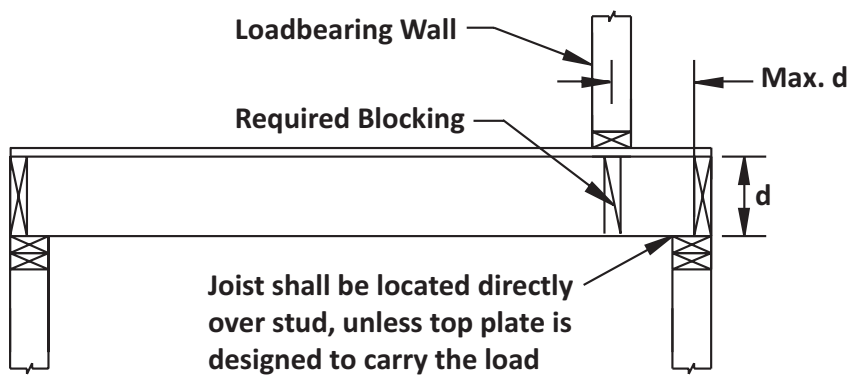
Figure 2.1d Setback Limits for Loadbearing Wall (see 2.1.3.2d)
