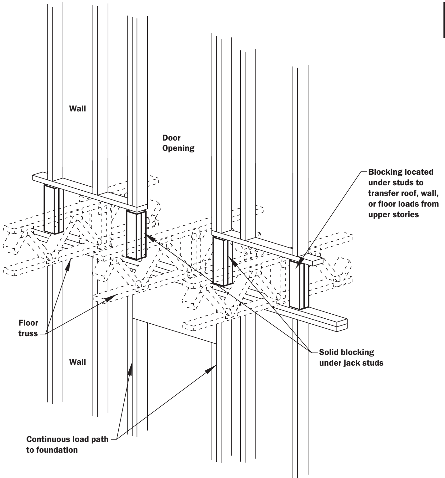
Figure 2.15b Blocking in Floor Space at Interior Loadbearing Walls
