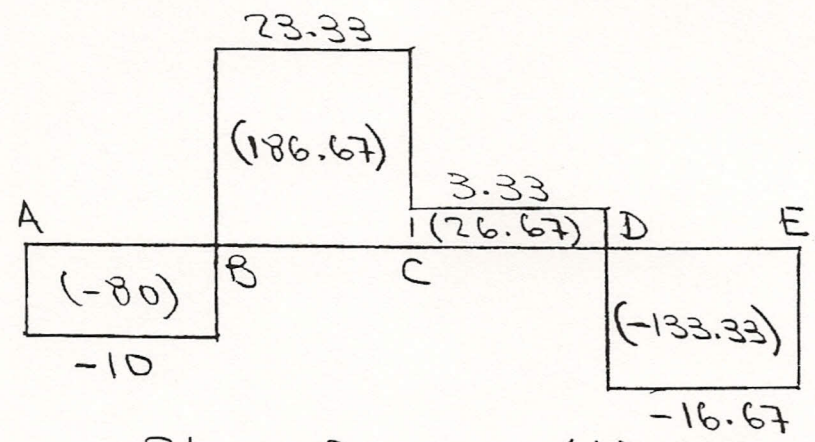
Shear Diagram (k)
