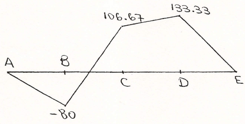
Bending Moment Diagram (k-ft)
