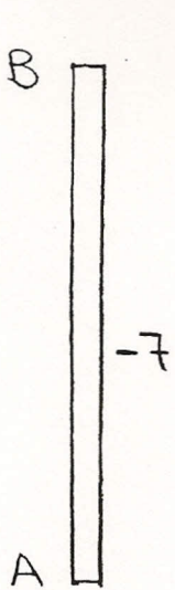
Axial Force Diagrams (k)
