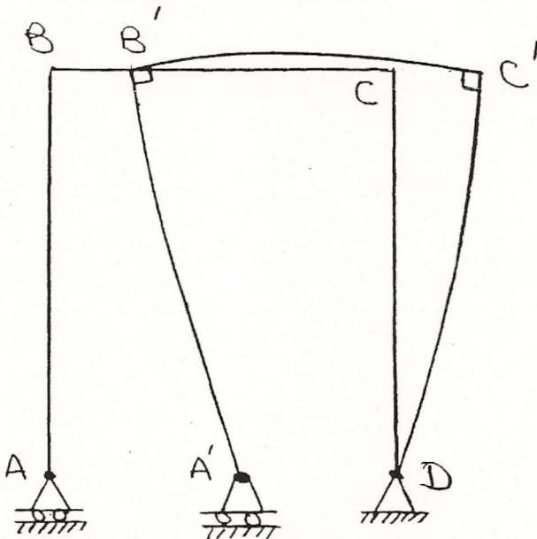
Qualitative Deflected Shape
