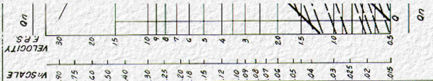
CHANNEL CHART 2:1 b = 5 FT.
