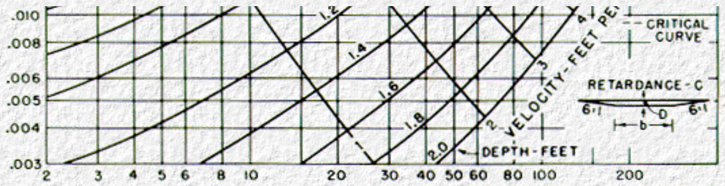
GRASSED CHANNELS 6:1 b = 4 ft.
