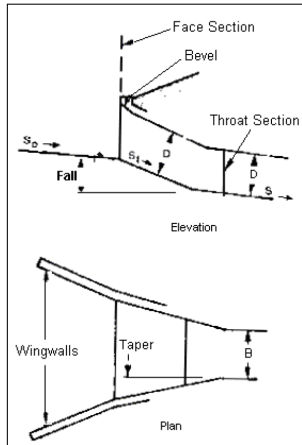
Figure I-10--Slope-tapered inlet
