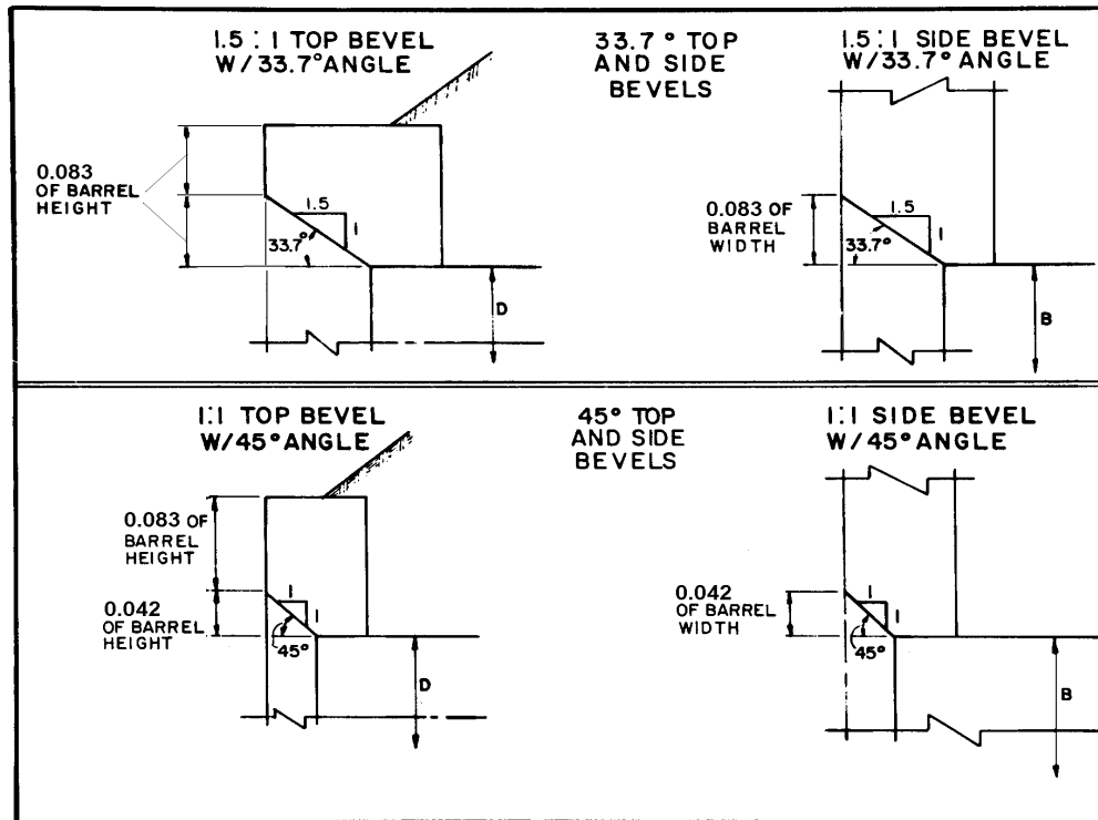
Figure III-3--Beveled Edges
