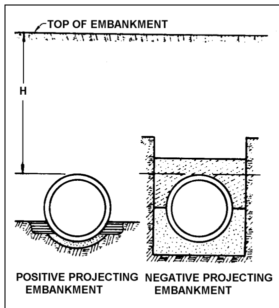
Figure VI-31--Culvert installation
