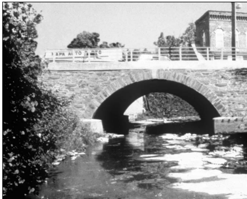
Figure VI-35--Long Span Culvert (Contech)
