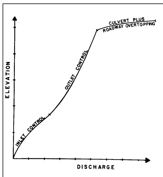
Figure V-5--Performance curve
