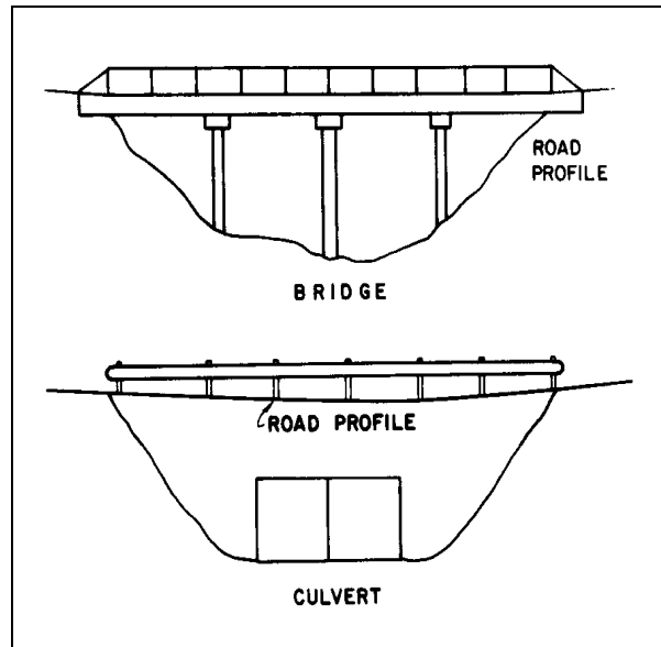
Figure VI-23--Bridge versus culvert at same location
