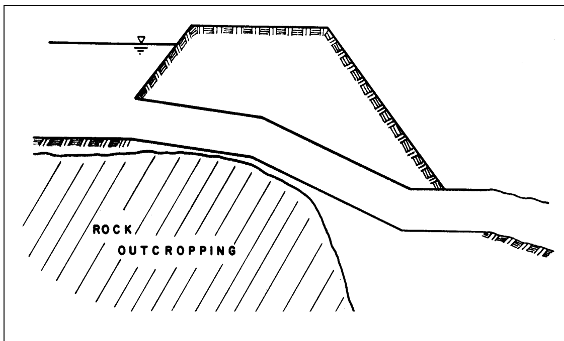
Figure VI-3--"Broken-Back" Culvert
