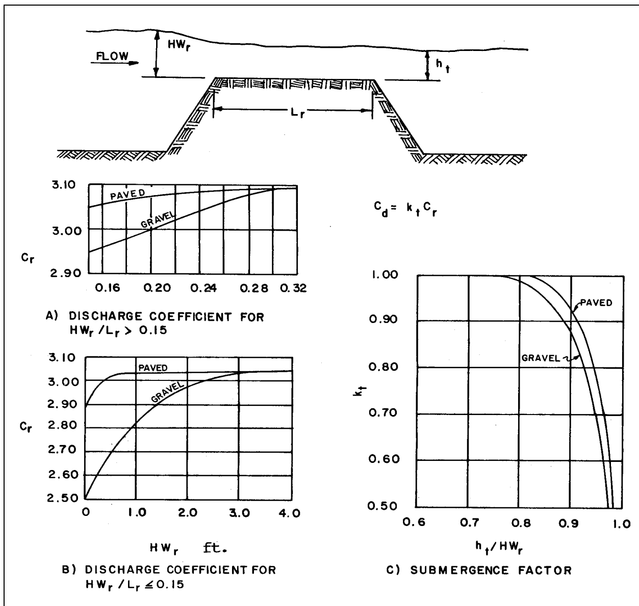
Figure III-11--English Discharge Coefficients for Roadway Overtopping
