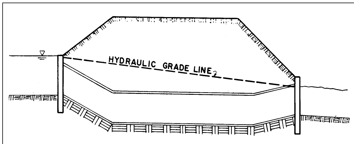
Figure VI-2--Sag Culvert
