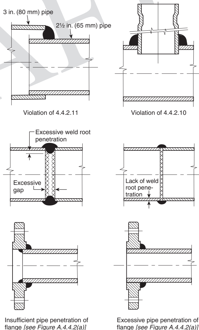
FIGURE A.4.4.2(b) Unacceptable Weld Joints. [13:Figure A.6.5.2(b)]
