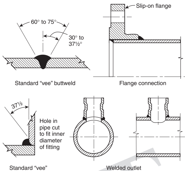
FIGURE A.4.4.2(a) Acceptable Weld Joints. [13:Figure A.6.5.2(a)]
