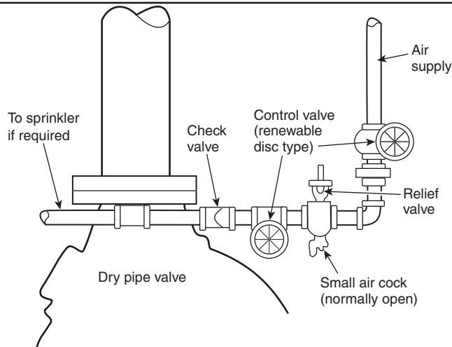
FIGURE 5.2.1.5.5 Air Supply from Shop System. [13:Figure 7.2.6.5]
