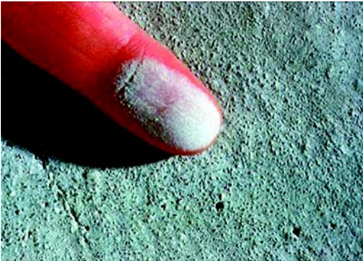
Fig. 2.2.9—Dusting.
