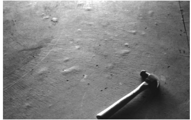
Fig. 2.3.2—Blistering.
