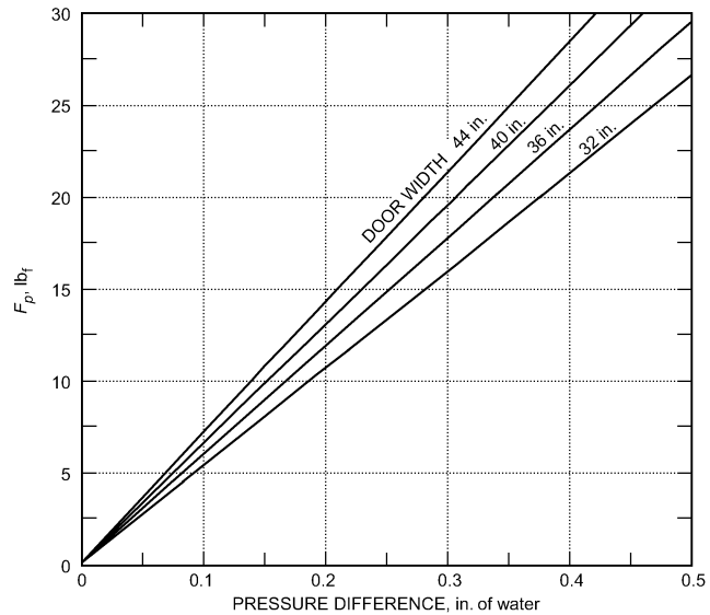
Fig. 7 Door-Opening Force Caused by Pressure Difference
