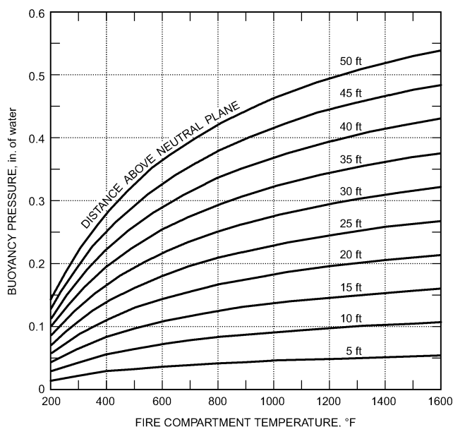
Fig. 5 Pressure Difference Caused by Buoyancy
