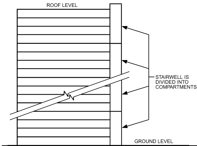
Fig. 14 Compartmentation of Pressurized Stairwell
