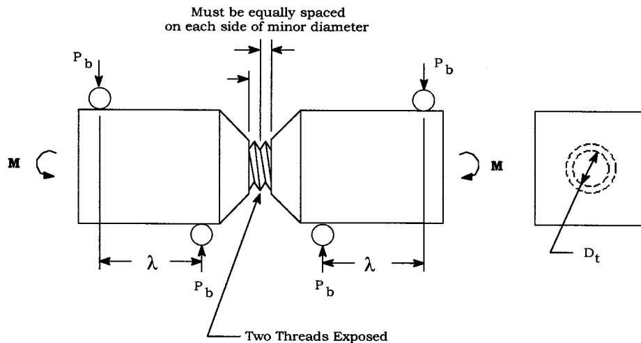
FIG. X1.1 Example of Test Method F 1624 Four Point Bend Test Fixtures
