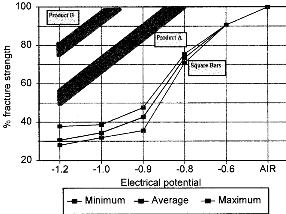
FIG. X1.2 Comparison of Threshold Data for Various Products and the Standard Square Bar Specimens for Alternate Threshold Determinations
