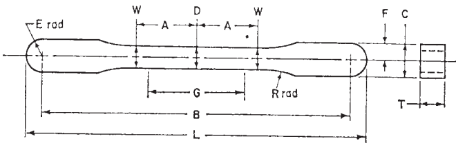
FIG. 18 Standard Tension Test Specimen for Die Castings
