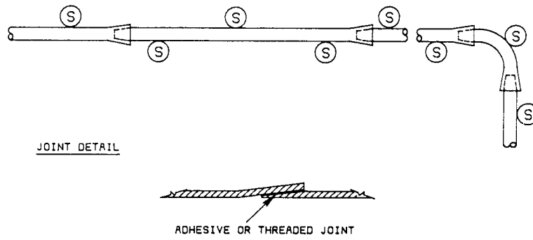
A3.2 Case II Bell and Spigot—Cemented or threaded joint system.
