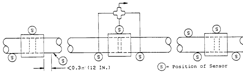
FIG. 1 Typical Sensor Positioning for Zone Location
