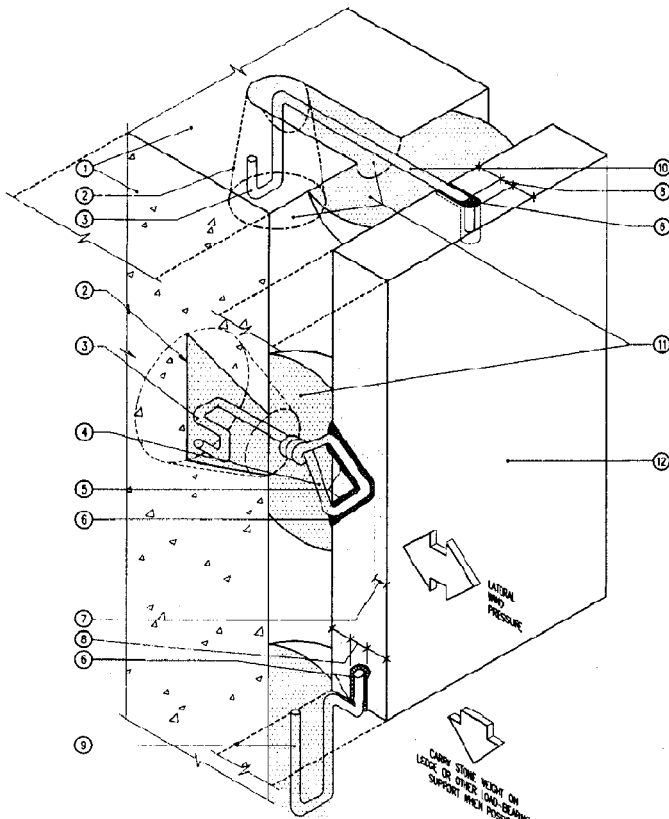
FIG. 9 Wire Ties
