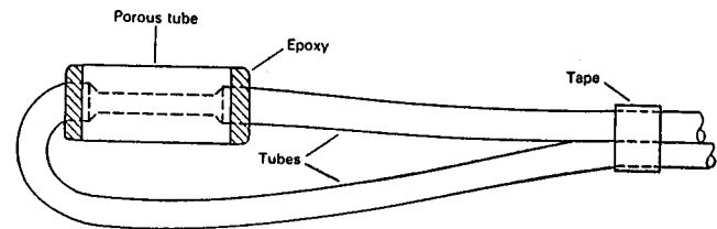
FIG. 3 Porous-Cup and Tube Designs
