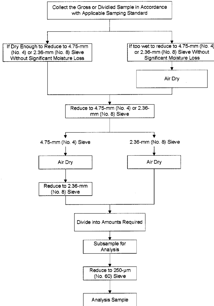
FIG. 3 Gross Sample Preparation Flowchart
