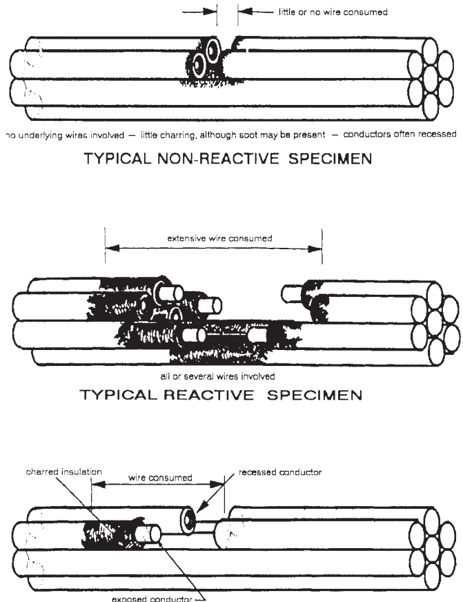
FIG. 28 Specimen Measurements
