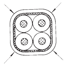
FIG. 11 Shielded and Jacketed Twisted Quad
