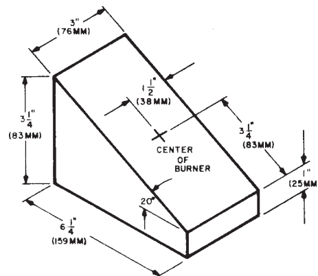
FIG. 14 Wedge Block
