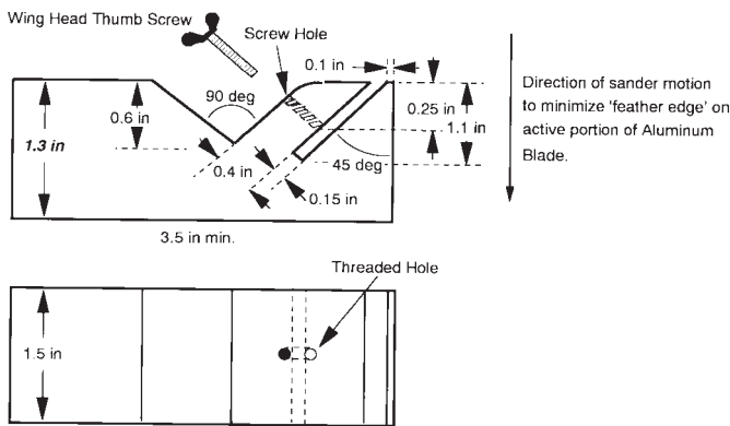
FIG. 27 Aluminum Blade Shaping Fixture
