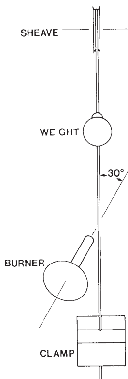
FIG. 17 Relative Positions of Burner and Specimen as Viewed as From the Right Side of the Enclosure
