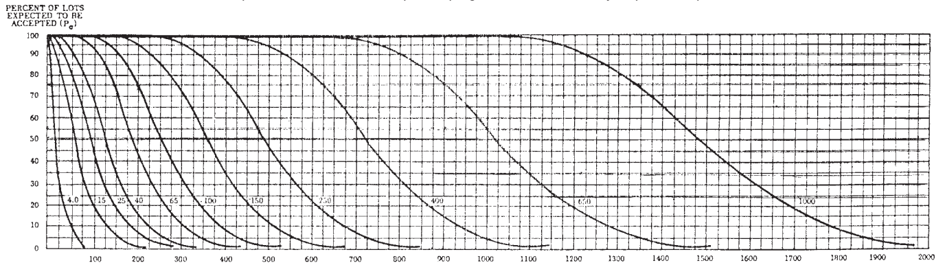
CHART B—OPERATING CHARACTERISTIC CURVES FOR SINGLE SAMPLING PLANS (Curves for double and multiple sampling are matched as closely as practicable)
