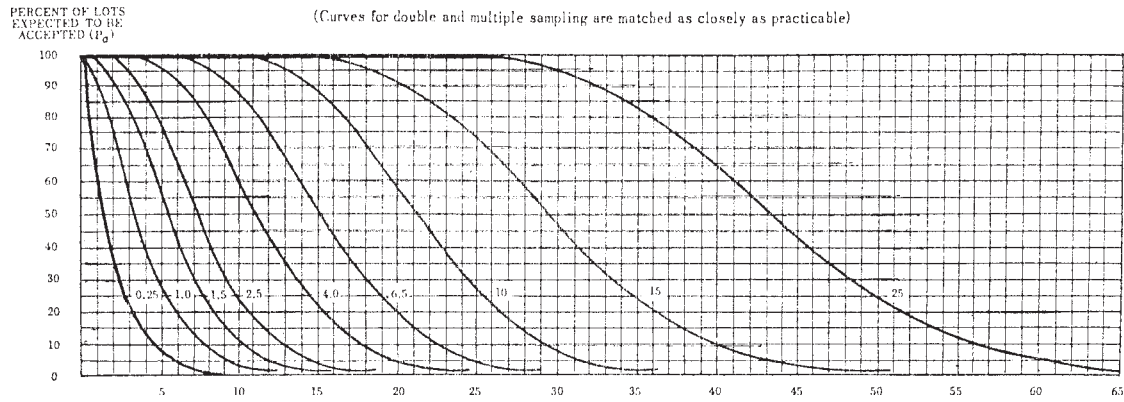
CHART H - OPERATING CHARACTERISTIC CURVES FOR SINGLE SAMPLING PLANS
