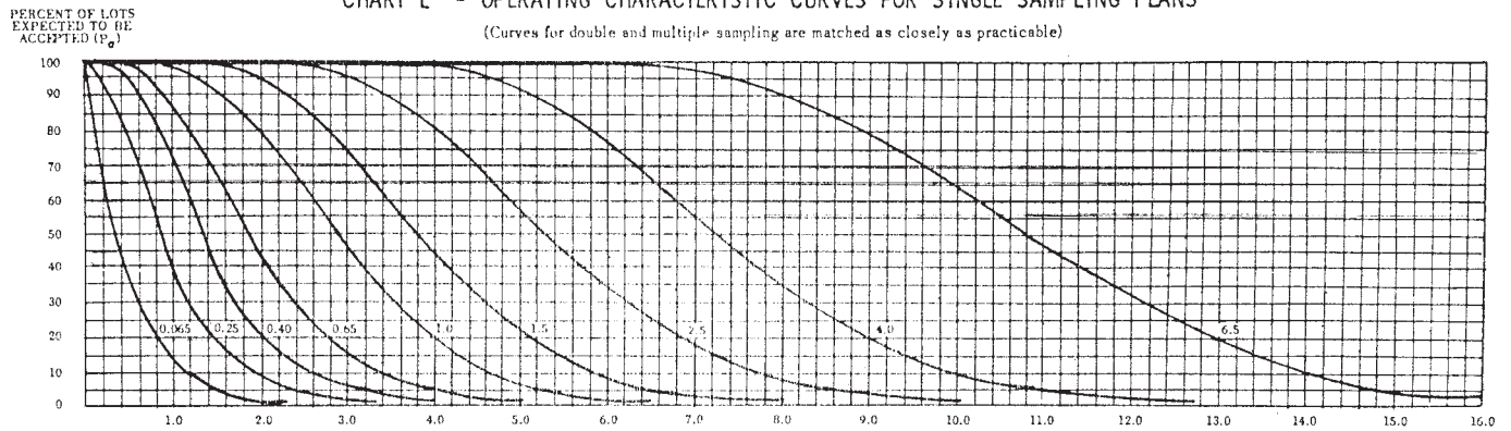
CHART L - OPERATING CHARACTERISTIC CURVES FOR SINGLE SAMPLING PLANS
