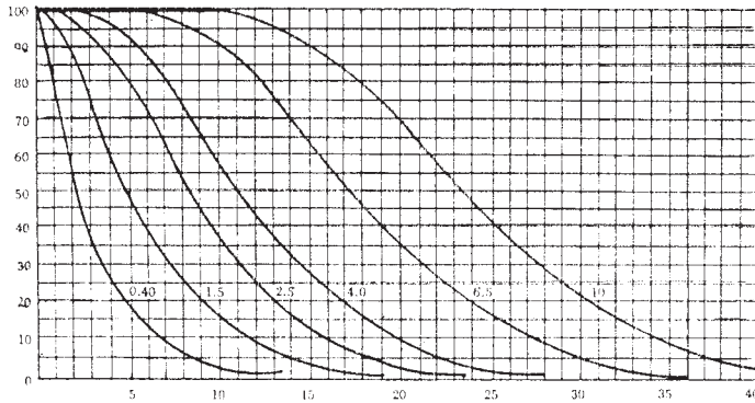
CHART G - OPERATING CHARACTERISTIC CURVES FOR SINGLE SAMPLING PLANS
