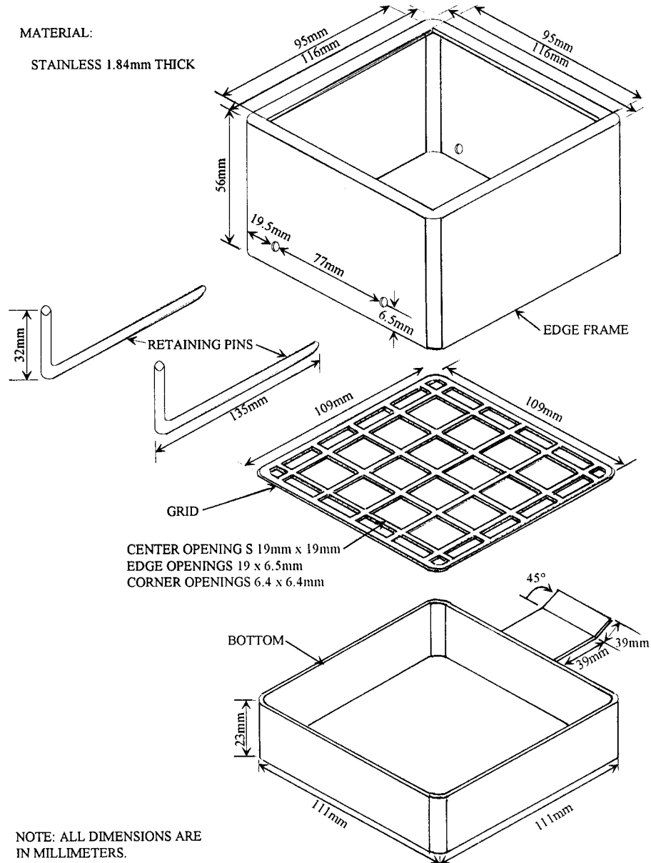
FIG. 1 Specimen Holder
