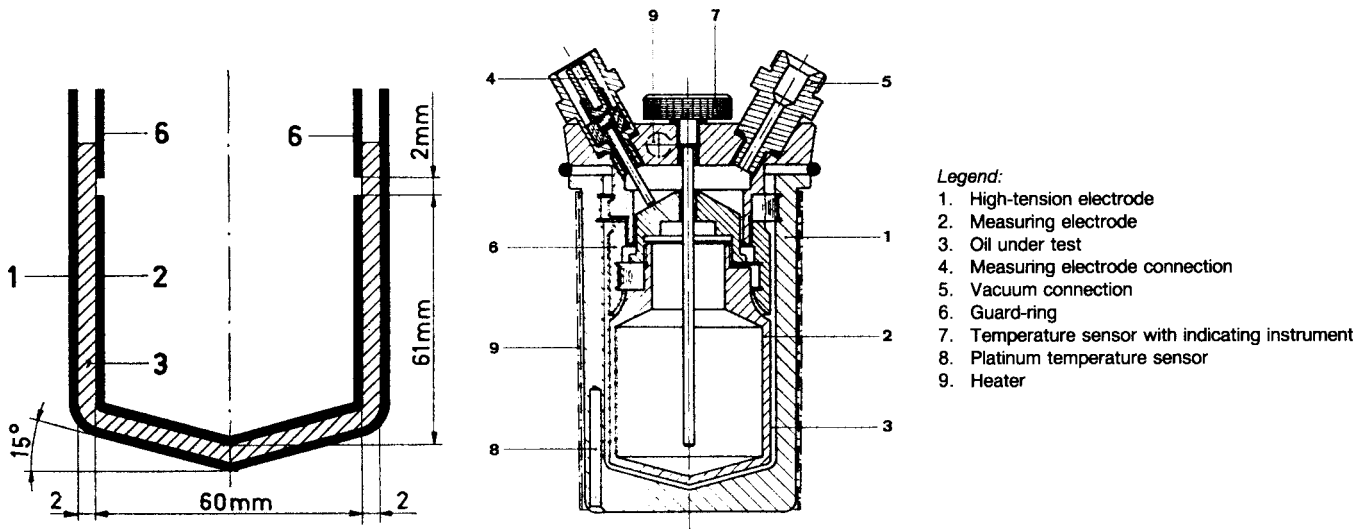
FIG. A1.3 Test Cell
