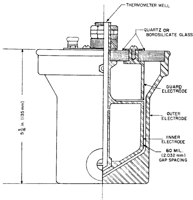
FIG. A1.1 Cell for Referee Tests
