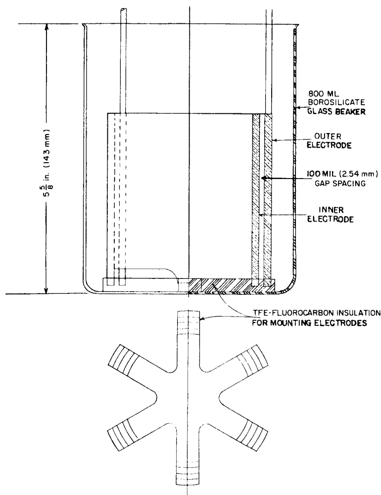
FIG. A1.4 Two-Electrode Cell for Routine Tests
