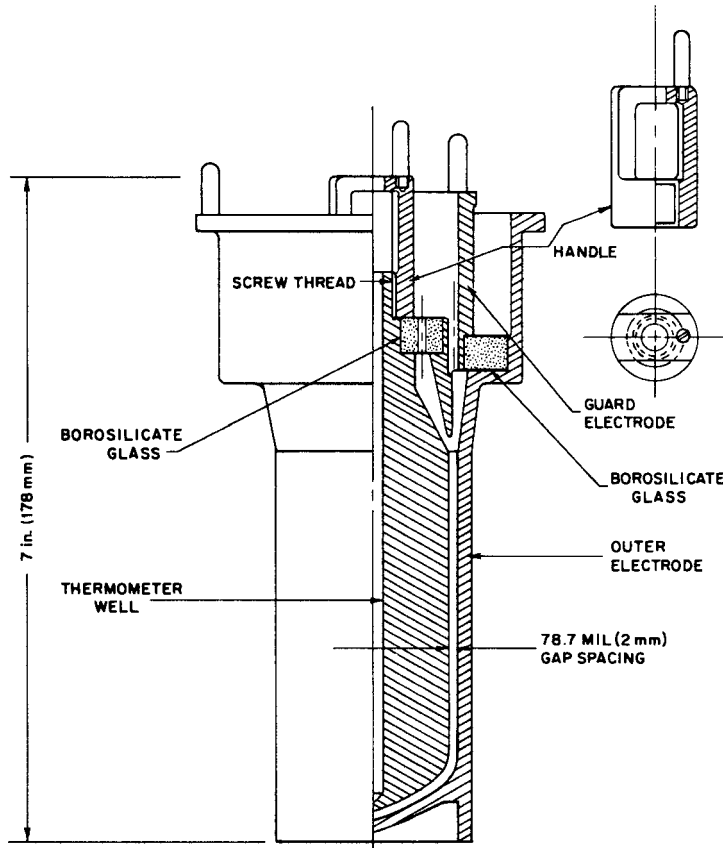
FIG. A1.2 Small-Capacity Cell for Referee Tests and Research Investigations
